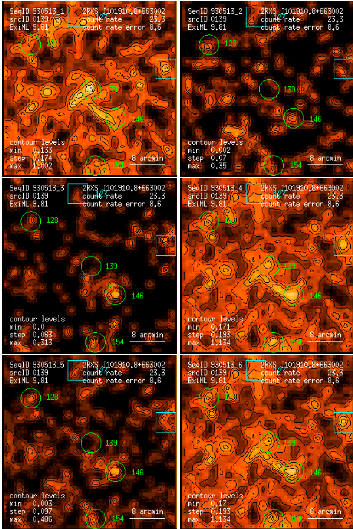
Figure 139: RASS 930513: detection 0139: band rate images, Gaussian filter: (1) PSPC channels 11 – 41, (2) 52 – 90, (3) 91 – 201, (4) 11 – 235, (5) 52 – 201, (6) 11 – 201. Broad band rates in counts/ks. Band rate contour levels in counts/ks/arcmin 2 .
