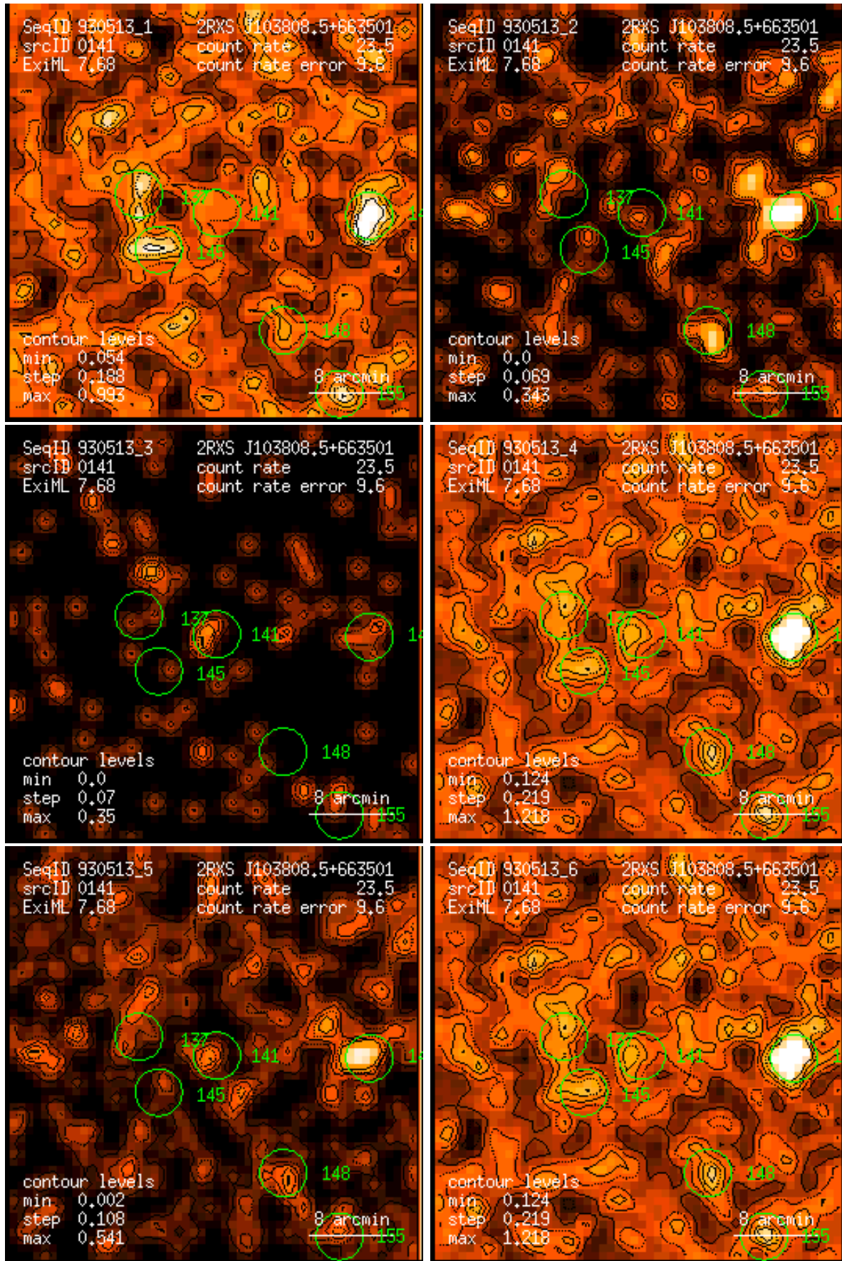
Figure 141: RASS 930513: detection 0141: band rate images, Gaussian filter: (1) PSPC channels 11 – 41, (2) 52 – 90, (3) 91 – 201, (4) 11 – 235, (5) 52 – 201, (6) 11 – 201. Broad band rates in counts/ks. Band rate contour levels in counts/ks/arcmin 2 .
