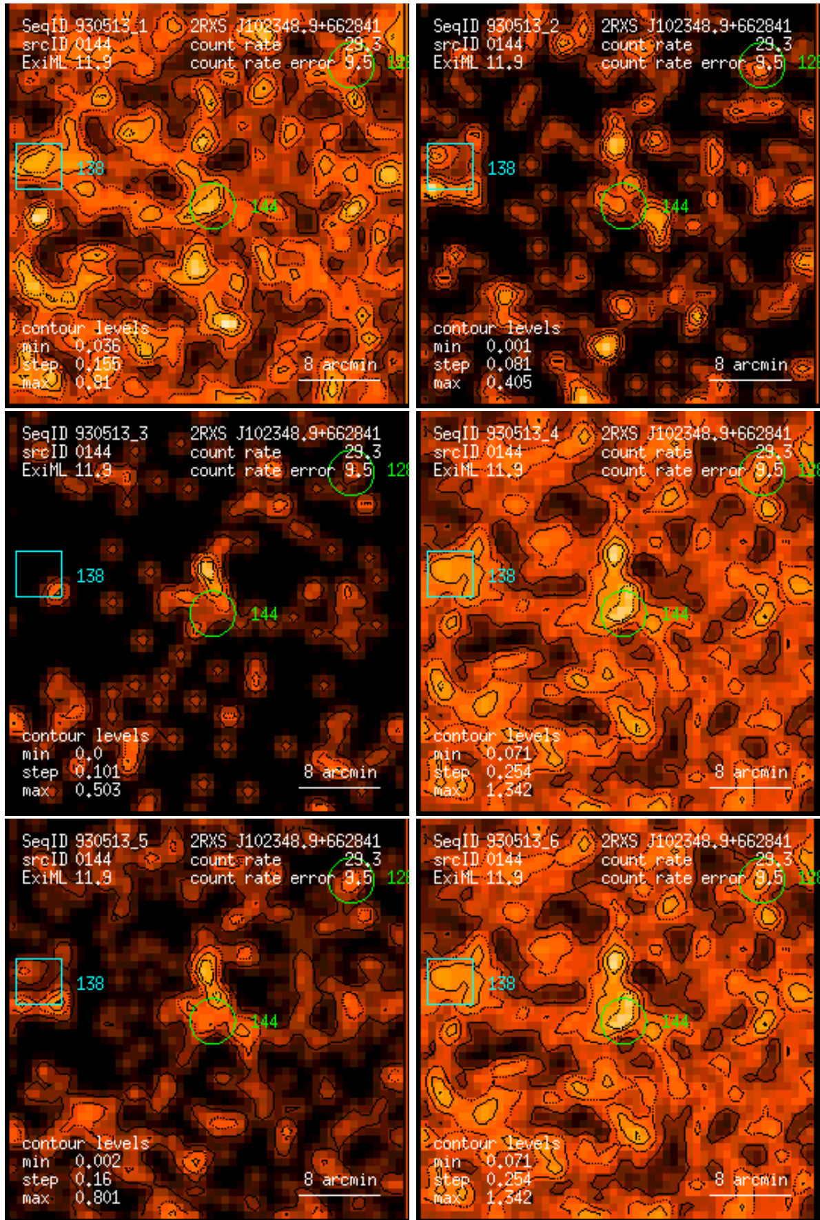
Figure 144: RASS 930513: detection 0144: band rate images, Gaussian filter: (1) PSPC channels 11 – 41, (2) 52 – 90, (3) 91 – 201, (4) 11 – 235, (5) 52 – 201, (6) 11 – 201. Broad band rates in counts/ks. Band rate contour levels in counts/ks/arcmin 2 .
