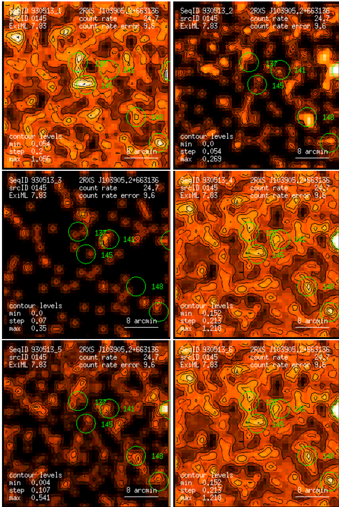
Figure 145: RASS 930513: detection 0145: band rate images, Gaussian filter: (1) PSPC channels 11 – 41, (2) 52 – 90, (3) 91 – 201, (4) 11 – 235, (5) 52 – 201, (6) 11 – 201. Broad band rates in counts/ks. Band rate contour levels in counts/ks/arcmin 2 .
