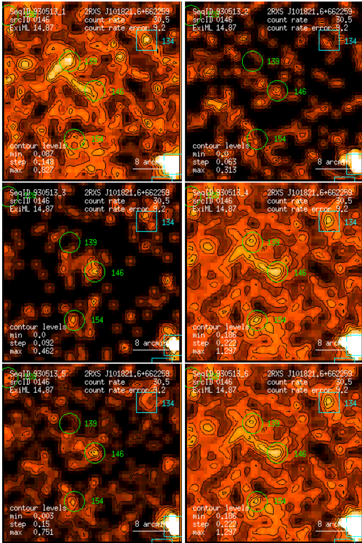
Figure 146: RASS 930513: detection 0146: band rate images, Gaussian filter: (1) PSPC channels 11 – 41, (2) 52 – 90, (3) 91 – 201, (4) 11 – 235, (5) 52 – 201, (6) 11 – 201. Broad band rates in counts/ks. Band rate contour levels in counts/ks/arcmin 2 .
