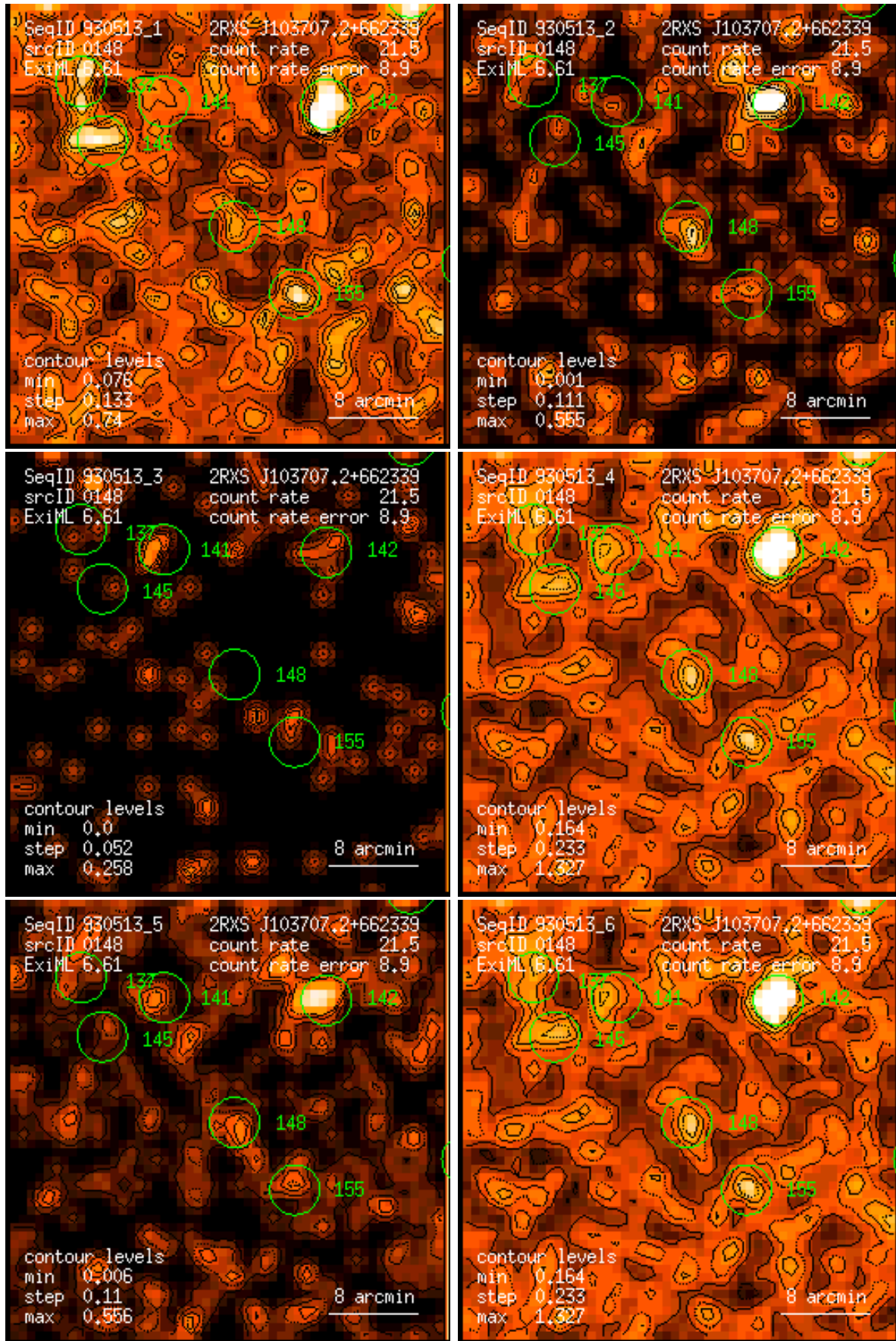
Figure 148: RASS 930513: detection 0148: band rate images, Gaussian filter: (1) PSPC channels 11 – 41, (2) 52 – 90, (3) 91 – 201, (4) 11 – 235, (5) 52 – 201, (6) 11 – 201. Broad band rates in counts/ks. Band rate contour levels in counts/ks/arcmin 2 .
