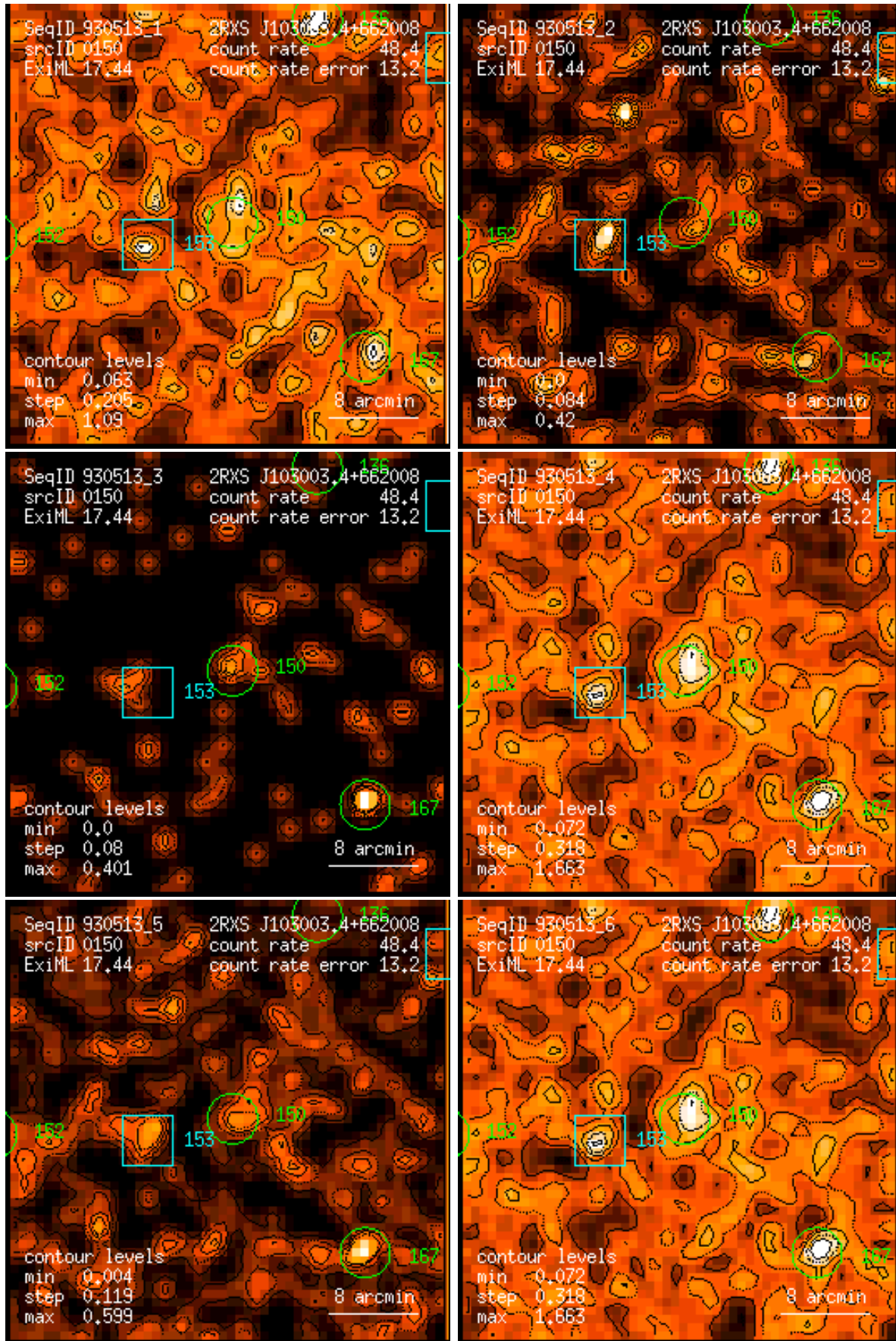
Figure 150: RASS 930513: detection 0150: band rate images, Gaussian filter: (1) PSPC channels 11 – 41, (2) 52 – 90, (3) 91 – 201, (4) 11 – 235, (5) 52 – 201, (6) 11 – 201. Broad band rates in counts/ks. Band rate contour levels in counts/ks/arcmin 2 .
