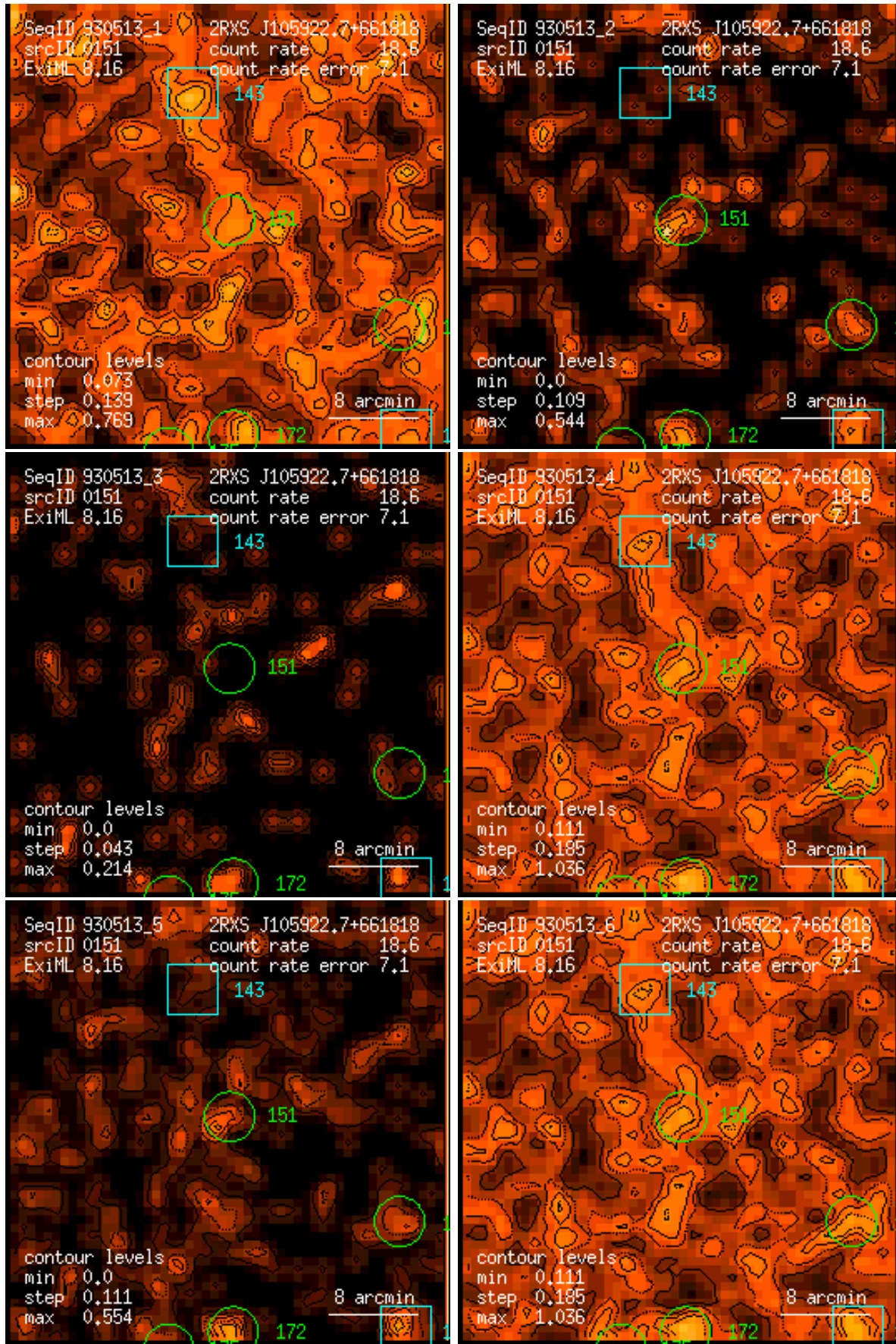
Figure 151: RASS 930513: detection 0151: band rate images, Gaussian filter: (1) PSPC channels 11 – 41, (2) 52 – 90, (3) 91 – 201, (4) 11 – 235, (5) 52 – 201, (6) 11 – 201. Broad band rates in counts/ks. Band rate contour levels in counts/ks/arcmin 2 .
