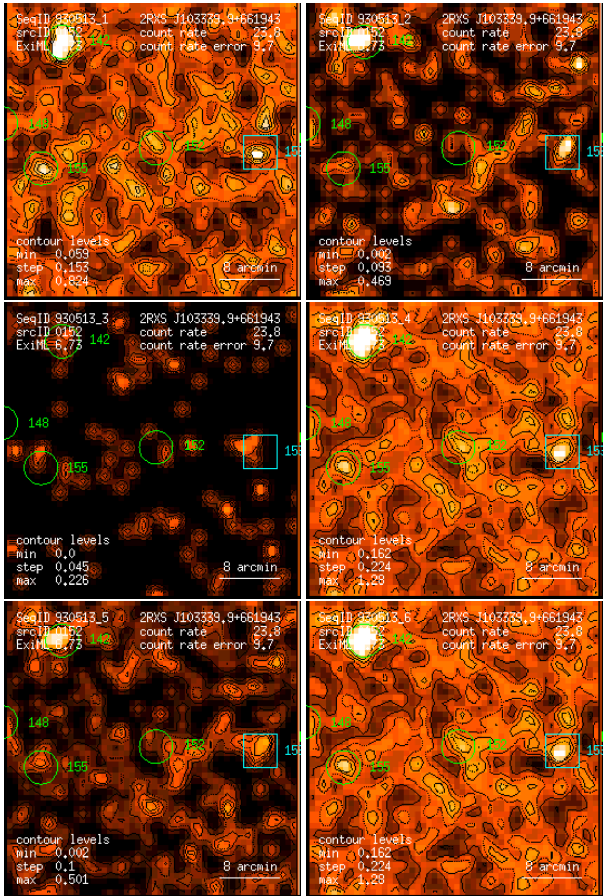
Figure 152: RASS 930513: detection 0152: band rate images, Gaussian filter: (1) PSPC channels 11 – 41, (2) 52 – 90, (3) 91 – 201, (4) 11 – 235, (5) 52 – 201, (6) 11 – 201. Broad band rates in counts/ks. Band rate contour levels in counts/ks/arcmin 2 .
