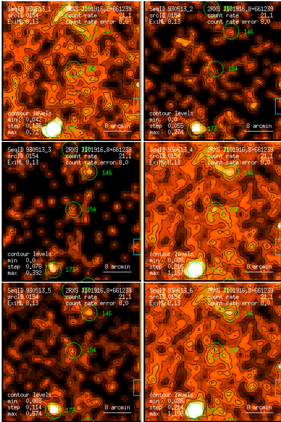
Figure 154: RASS 930513: detection 0154: band rate images, Gaussian filter: (1) PSPC channels 11 – 41, (2) 52 – 90, (3) 91 – 201, (4) 11 – 235, (5) 52 – 201, (6) 11 – 201. Broad band rates in counts/ks. Band rate contour levels in counts/ks/arcmin 2 .
