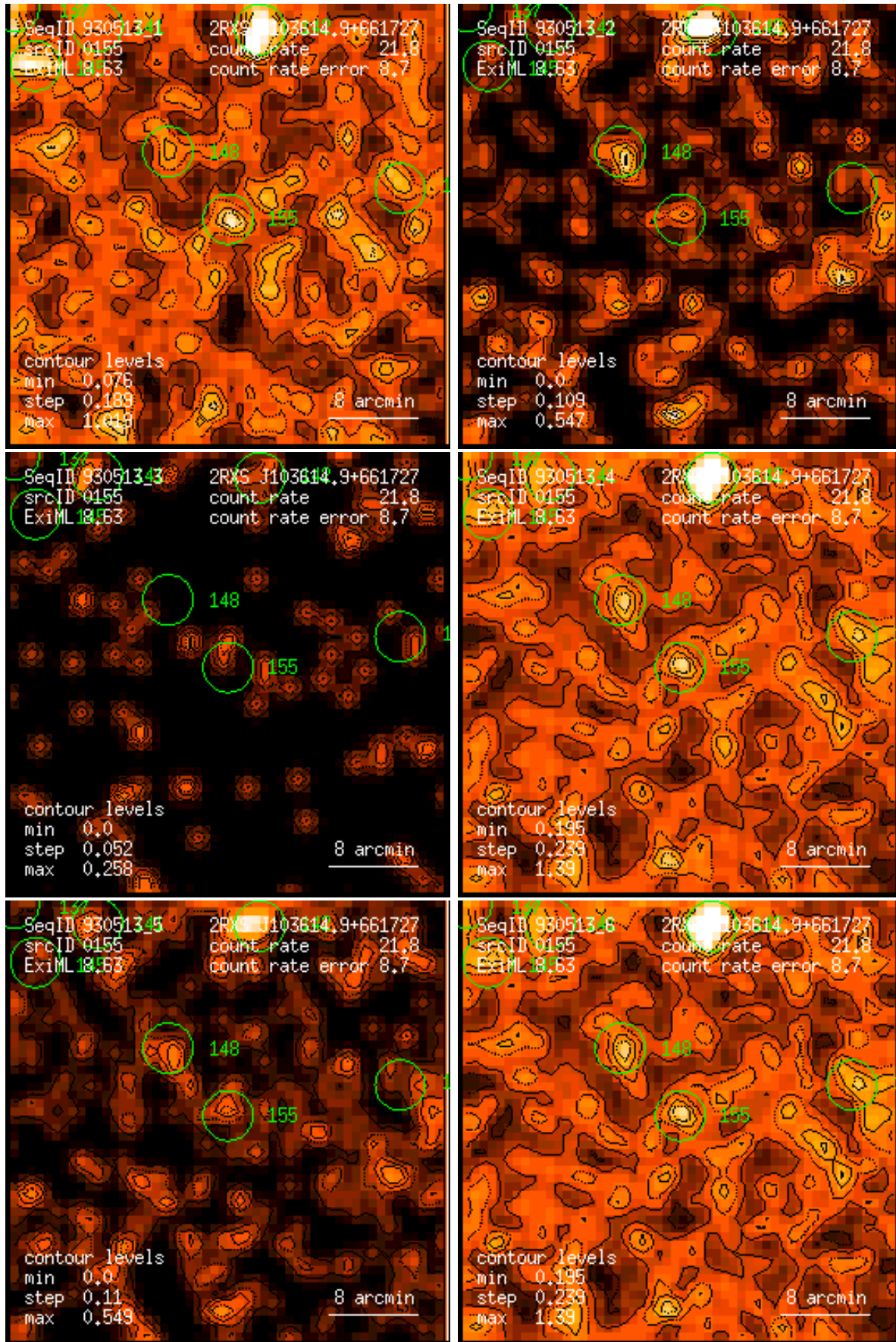
Figure 155: RASS 930513: detection 0155: band rate images, Gaussian filter: (1) PSPC channels 11 – 41, (2) 52 – 90, (3) 91 – 201, (4) 11 – 235, (5) 52 – 201, (6) 11 – 201. Broad band rates in counts/ks. Band rate contour levels in counts/ks/arcmin 2 .
