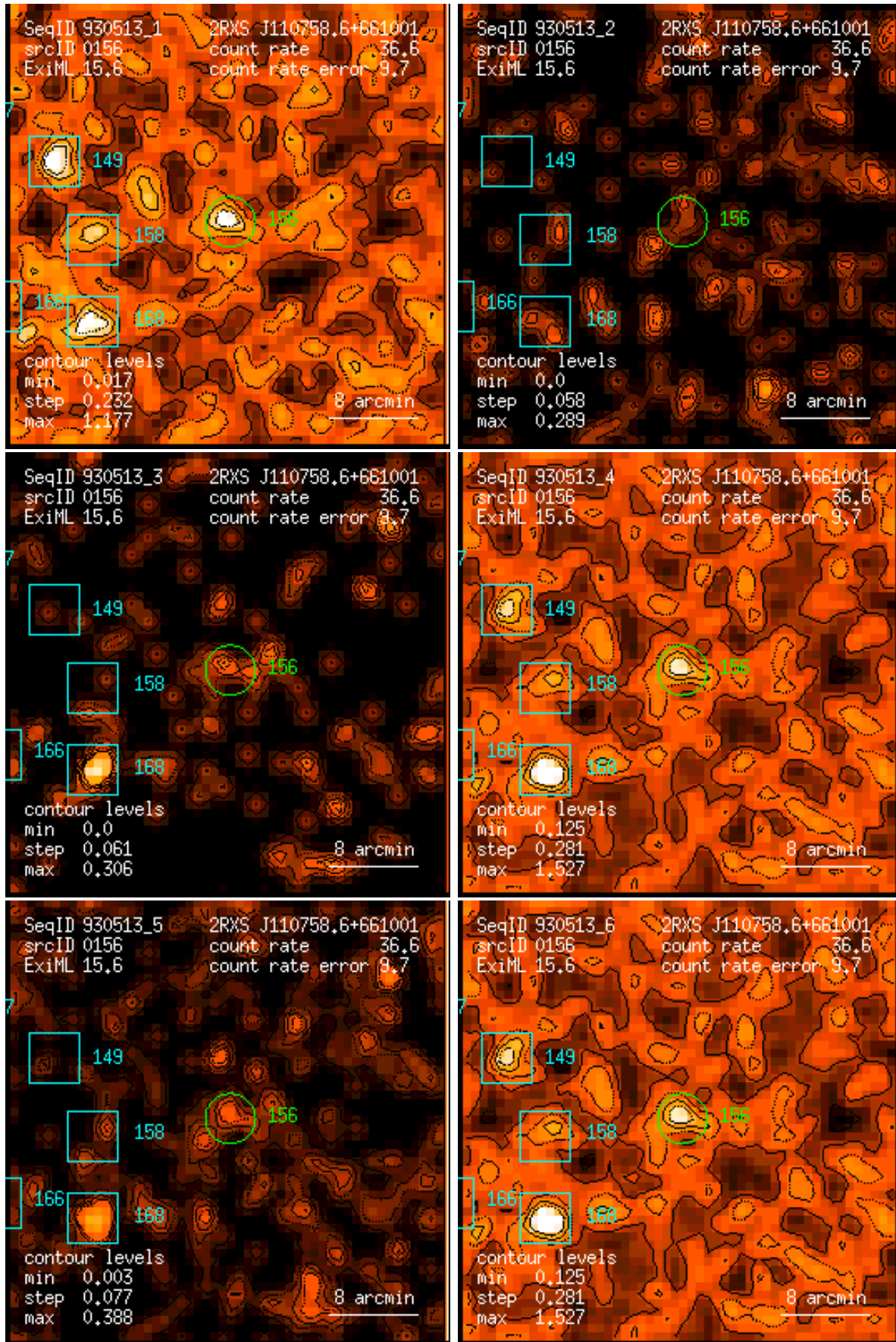
Figure 156: RASS 930513: detection 0156: band rate images, Gaussian filter: (1) PSPC channels 11 – 41, (2) 52 – 90, (3) 91 – 201, (4) 11 – 235, (5) 52 – 201, (6) 11 – 201. Broad band rates in counts/ks. Band rate contour levels in counts/ks/arcmin 2 .
