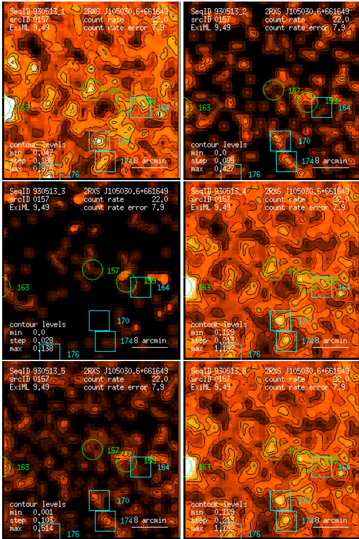
Figure 157: RASS 930513: detection 0157: band rate images, Gaussian filter: (1) PSPC channels 11 – 41, (2) 52 – 90, (3) 91 – 201, (4) 11 – 235, (5) 52 – 201, (6) 11 – 201. Broad band rates in counts/ks. Band rate contour levels in counts/ks/arcmin 2 .
