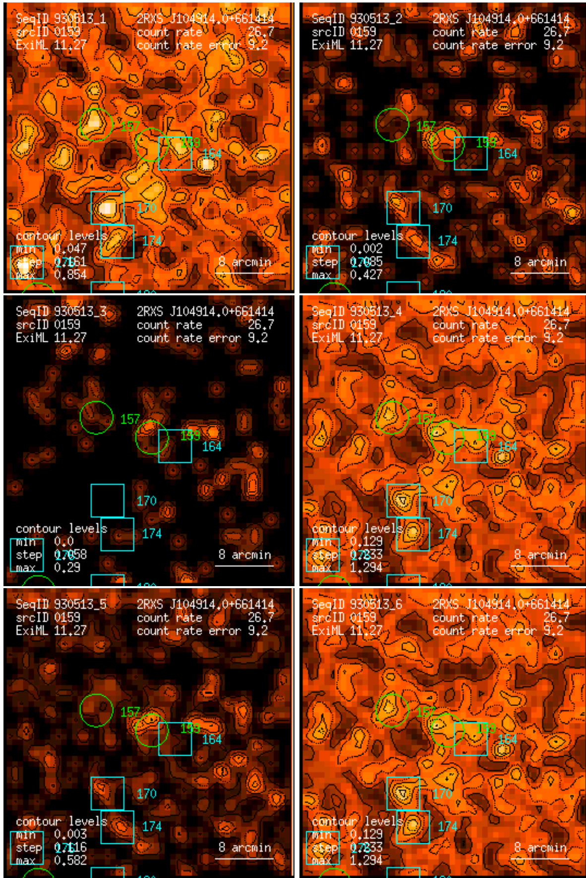
Figure 159: RASS 930513: detection 0159: band rate images, Gaussian filter: (1) PSPC channels 11 – 41, (2) 52 – 90, (3) 91 – 201, (4) 11 – 235, (5) 52 – 201, (6) 11 – 201. Broad band rates in counts/ks. Band rate contour levels in counts/ks/arcmin 2 .
