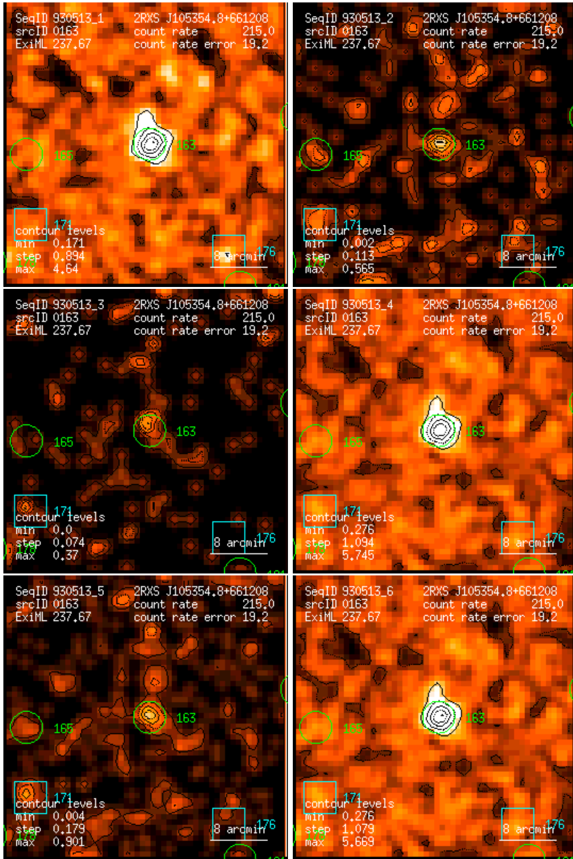
Figure 163: RASS 930513: detection 0163: band rate images, Gaussian filter: (1) PSPC channels 11 – 41, (2) 52 – 90, (3) 91 – 201, (4) 11 – 235, (5) 52 – 201, (6) 11 – 201. Broad band rates in counts/ks. Band rate contour levels in counts/ks/arcmin 2 .
