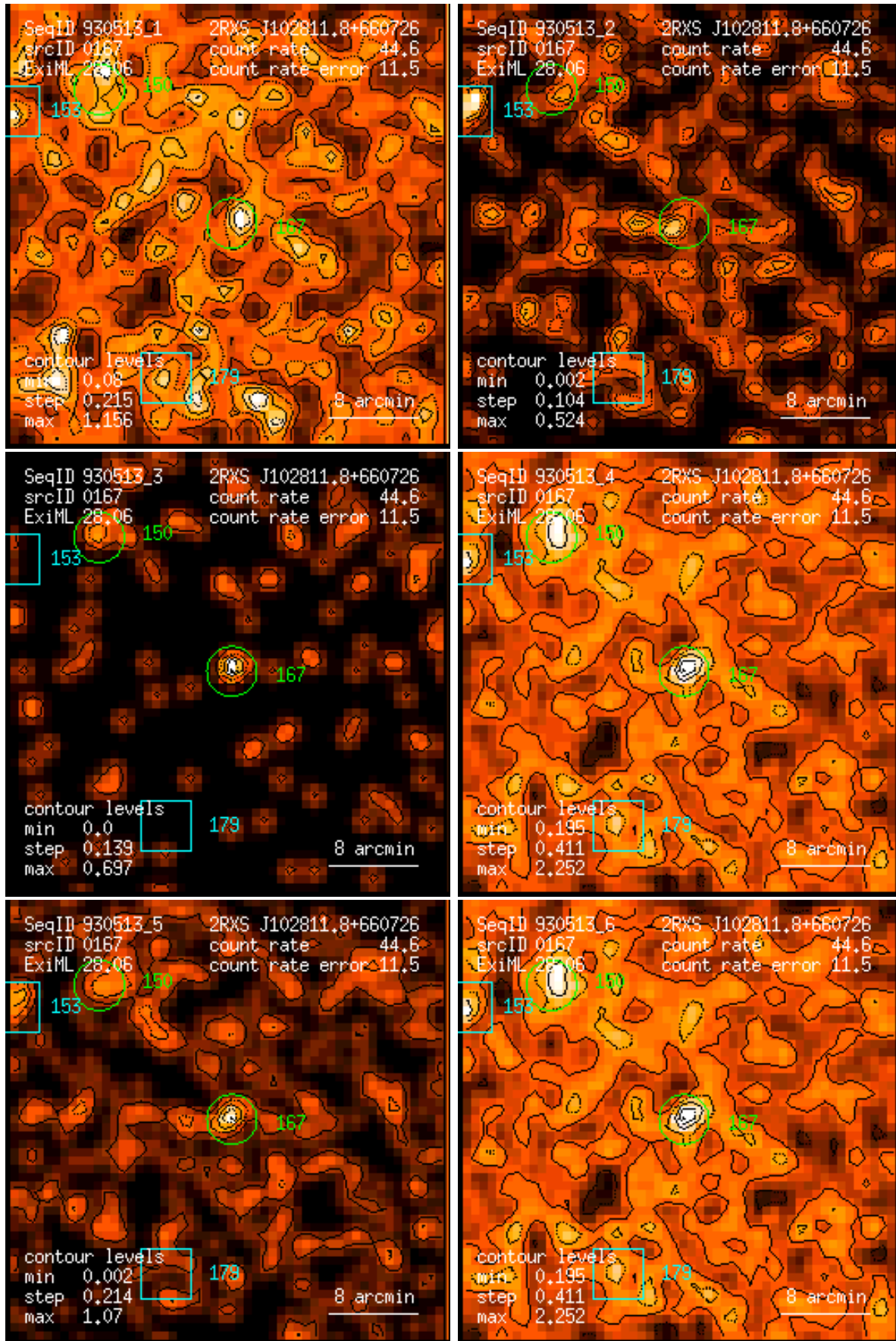
Figure 167: RASS 930513: detection 0167: band rate images, Gaussian filter: (1) PSPC channels 11 – 41, (2) 52 – 90, (3) 91 – 201, (4) 11 – 235, (5) 52 – 201, (6) 11 – 201. Broad band rates in counts/ks. Band rate contour levels in counts/ks/arcmin 2 .
