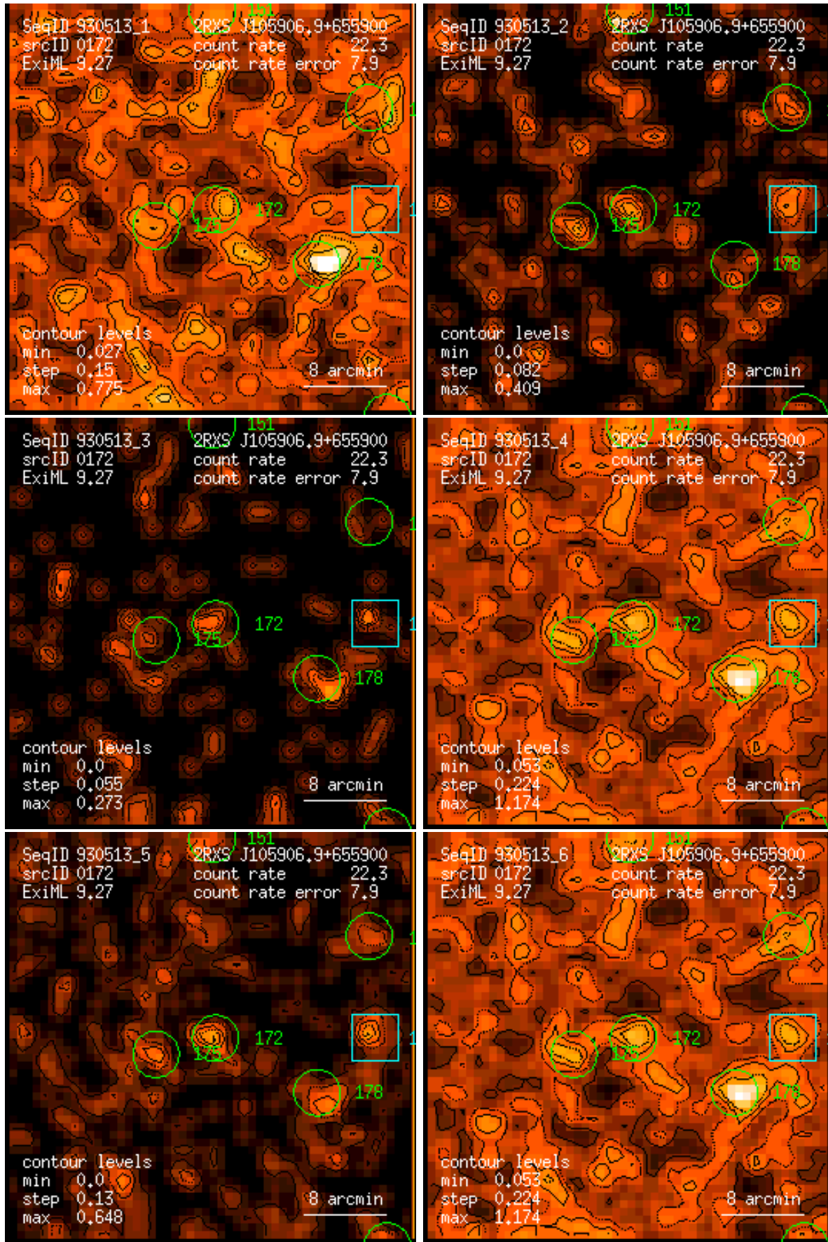
Figure 172: RASS 930513: detection 0172: band rate images, Gaussian filter: (1) PSPC channels 11 – 41, (2) 52 – 90, (3) 91 – 201, (4) 11 – 235, (5) 52 – 201, (6) 11 – 201. Broad band rates in counts/ks. Band rate contour levels in counts/ks/arcmin 2 .
