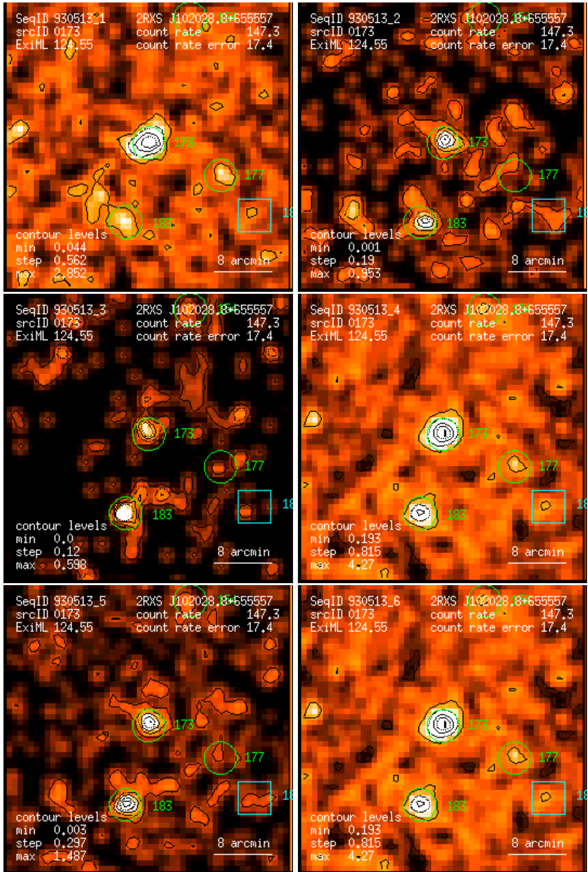
Figure 173: RASS 930513: detection 0173: band rate images, Gaussian filter: (1) PSPC channels 11 – 41, (2) 52 – 90, (3) 91 – 201, (4) 11 – 235, (5) 52 – 201, (6) 11 – 201. Broad band rates in counts/ks. Band rate contour levels in counts/ks/arcmin 2 .
