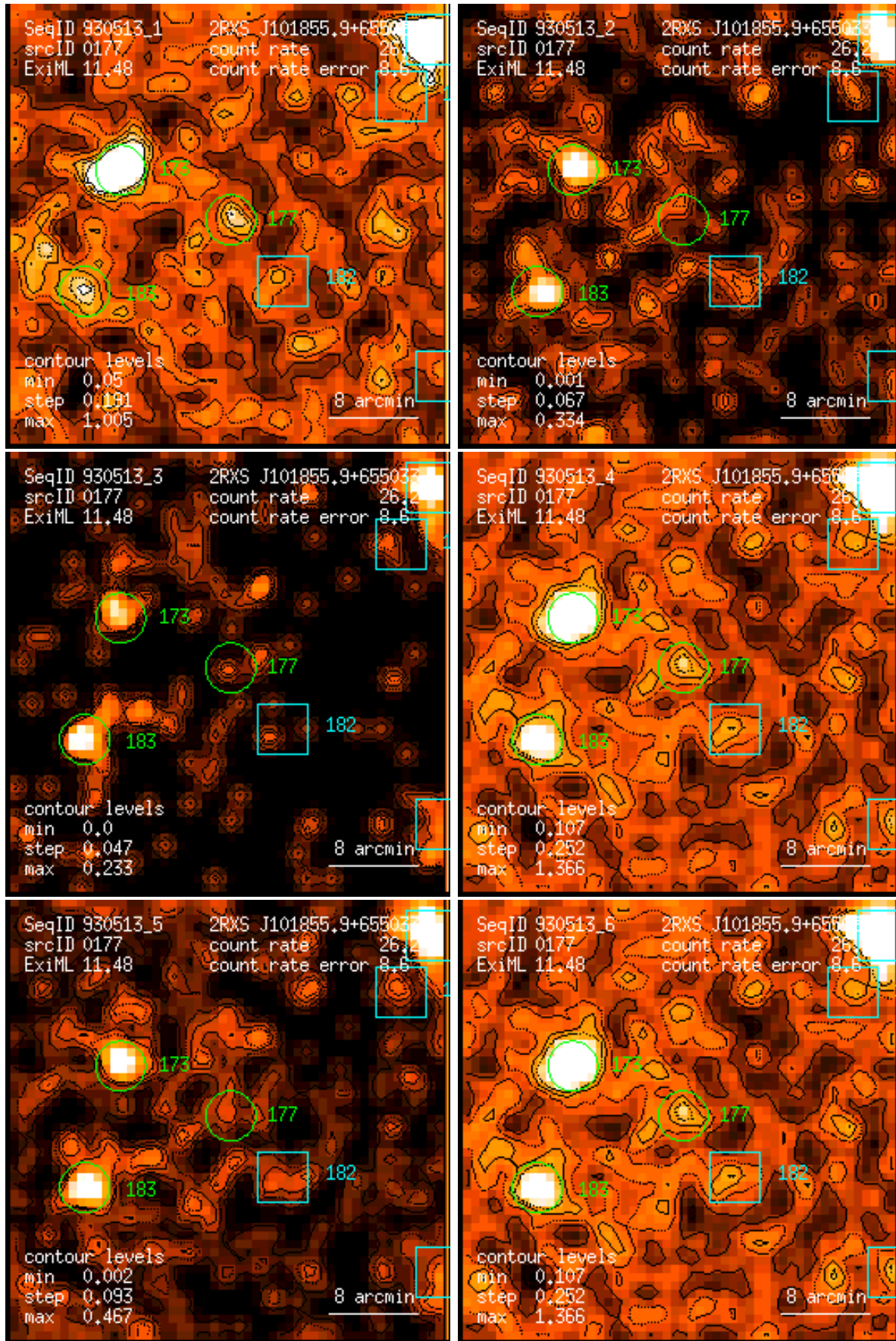
Figure 177: RASS 930513: detection 0177: band rate images, Gaussian filter: (1) PSPC channels 11 – 41, (2) 52 – 90, (3) 91 – 201, (4) 11 – 235, (5) 52 – 201, (6) 11 – 201. Broad band rates in counts/ks. Band rate contour levels in counts/ks/arcmin 2 .
