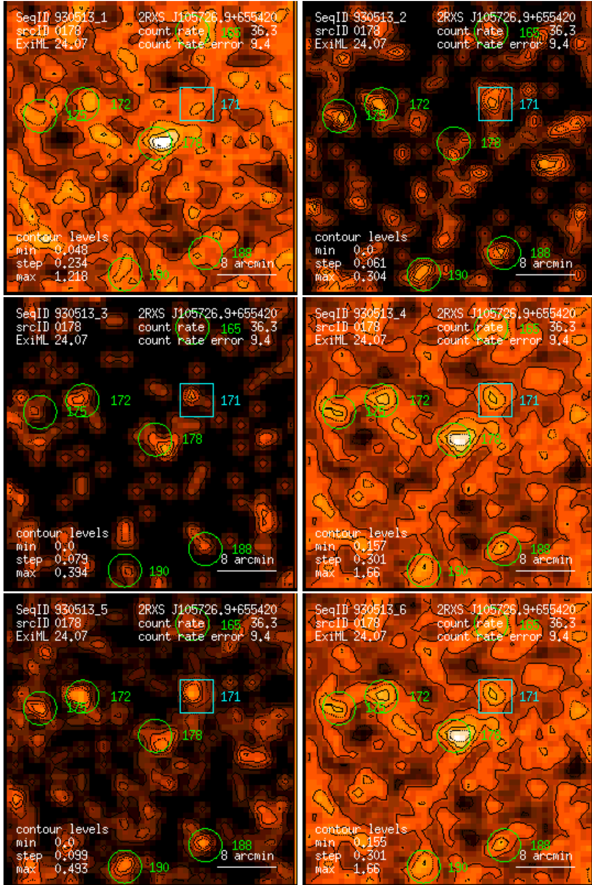
Figure 178: RASS 930513: detection 0178: band rate images, Gaussian filter: (1) PSPC channels 11 – 41, (2) 52 – 90, (3) 91 – 201, (4) 11 – 235, (5) 52 – 201, (6) 11 – 201. Broad band rates in counts/ks. Band rate contour levels in counts/ks/arcmin 2 .
