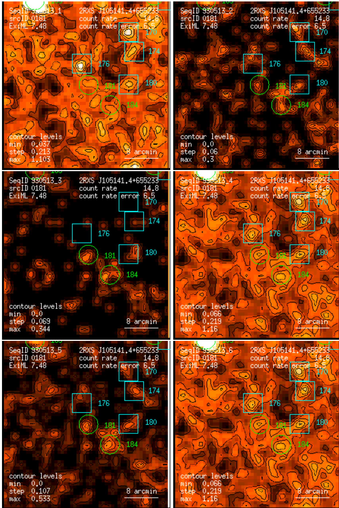
Figure 181: RASS 930513: detection 0181: band rate images, Gaussian filter: (1) PSPC channels 11 – 41, (2) 52 – 90, (3) 91 – 201, (4) 11 – 235, (5) 52 – 201, (6) 11 – 201. Broad band rates in counts/ks. Band rate contour levels in counts/ks/arcmin 2 .
