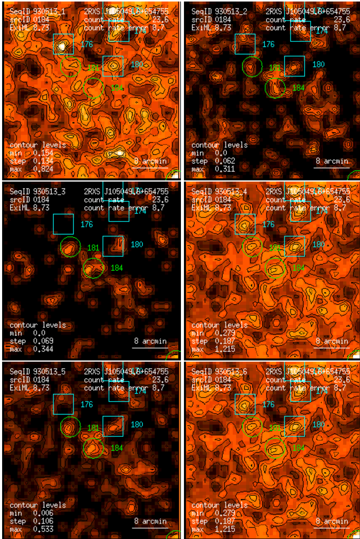
Figure 184: RASS 930513: detection 0184: band rate images, Gaussian filter: (1) PSPC channels 11 – 41, (2) 52 – 90, (3) 91 – 201, (4) 11 – 235, (5) 52 – 201, (6) 11 – 201. Broad band rates in counts/ks. Band rate contour levels in counts/ks/arcmin 2 .
