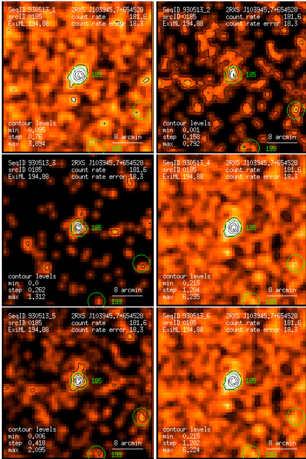
Figure 185: RASS 930513: detection 0185: band rate images, Gaussian filter: (1) PSPC channels 11 – 41, (2) 52 – 90, (3) 91 – 201, (4) 11 – 235, (5) 52 – 201, (6) 11 – 201. Broad band rates in counts/ks. Band rate contour levels in counts/ks/arcmin 2 .
