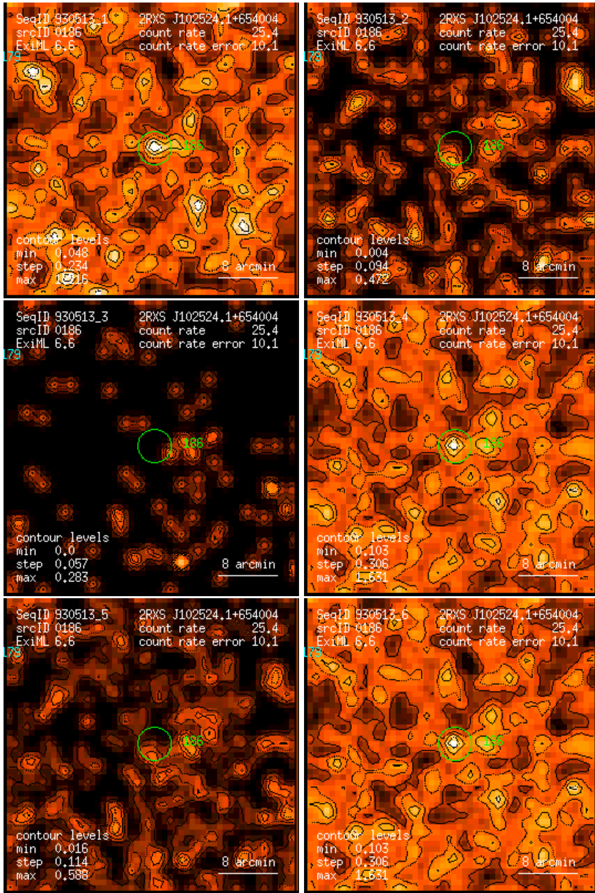
Figure 186: RASS 930513: detection 0186: band rate images, Gaussian filter: (1) PSPC channels 11 – 41, (2) 52 – 90, (3) 91 – 201, (4) 11 – 235, (5) 52 – 201, (6) 11 – 201. Broad band rates in counts/ks. Band rate contour levels in counts/ks/arcmin 2 .
