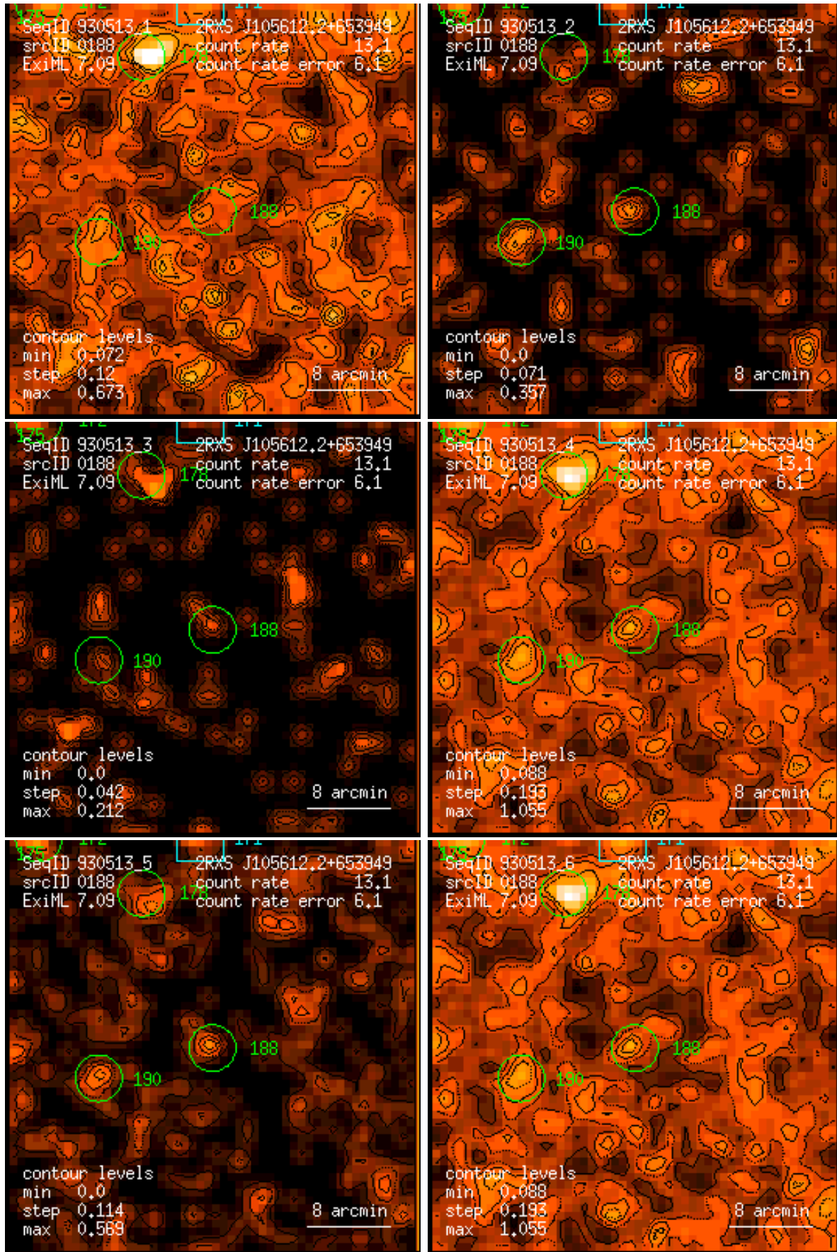
Figure 188: RASS 930513: detection 0188: band rate images, Gaussian filter: (1) PSPC channels 11 – 41, (2) 52 – 90, (3) 91 – 201, (4) 11 – 235, (5) 52 – 201, (6) 11 – 201. Broad band rates in counts/ks. Band rate contour levels in counts/ks/arcmin 2 .
