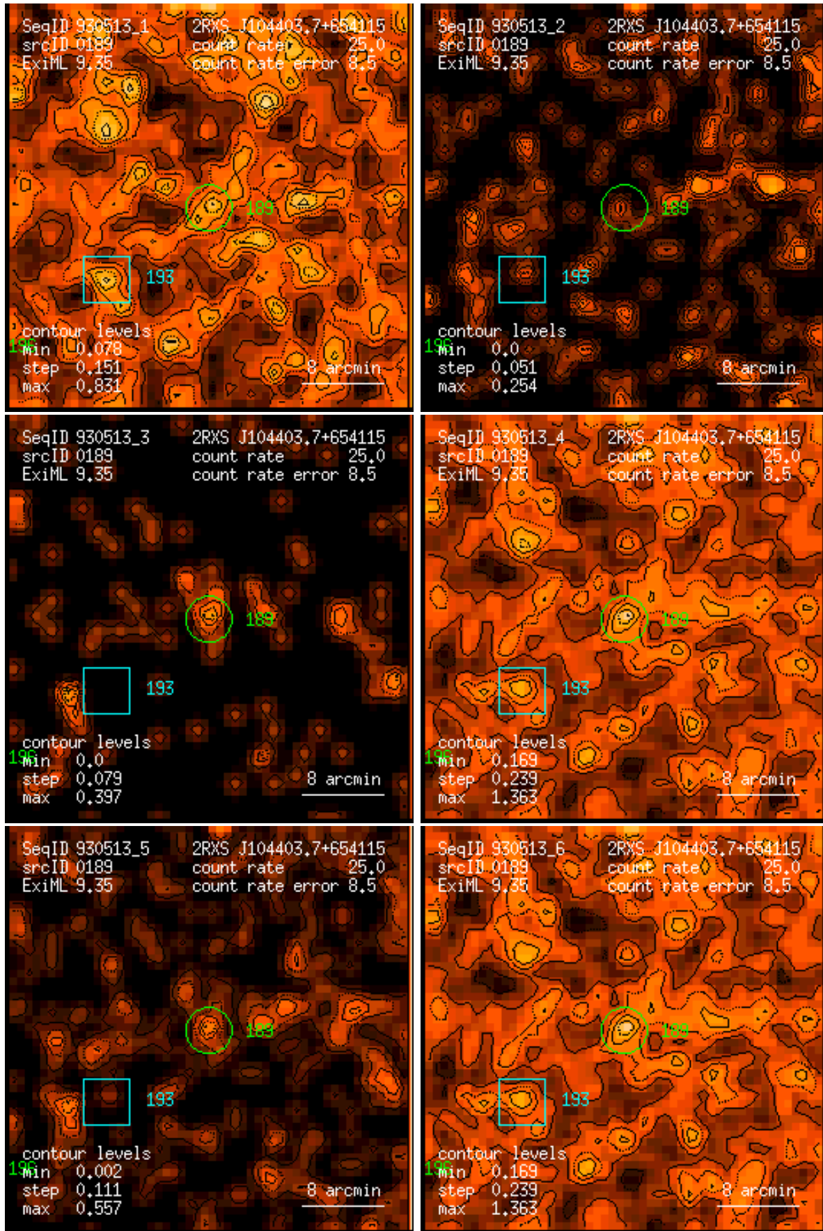
Figure 189: RASS 930513: detection 0189: band rate images, Gaussian filter: (1) PSPC channels 11 – 41, (2) 52 – 90, (3) 91 – 201, (4) 11 – 235, (5) 52 – 201, (6) 11 – 201. Broad band rates in counts/ks. Band rate contour levels in counts/ks/arcmin 2 .
