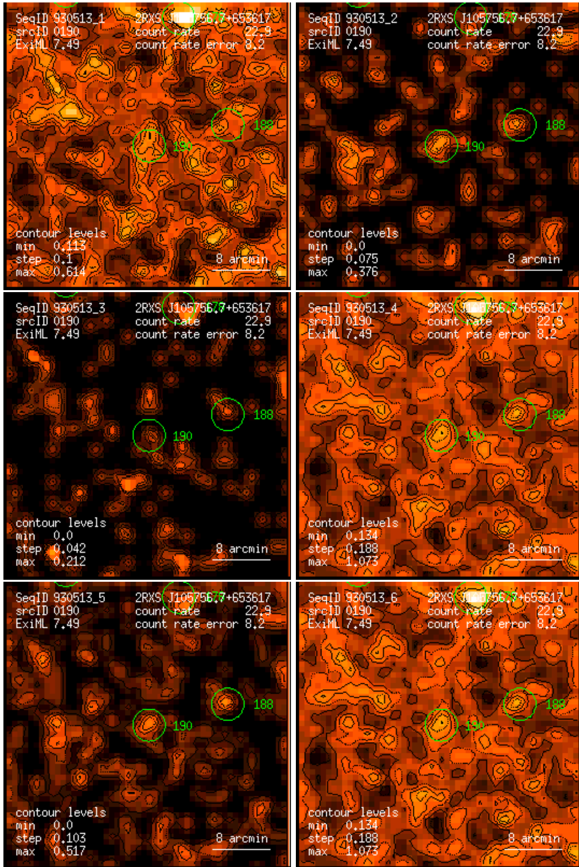
Figure 190: RASS 930513: detection 0190: band rate images, Gaussian filter: (1) PSPC channels 11 – 41, (2) 52 – 90, (3) 91 – 201, (4) 11 – 235, (5) 52 – 201, (6) 11 – 201. Broad band rates in counts/ks. Band rate contour levels in counts/ks/arcmin 2 .
