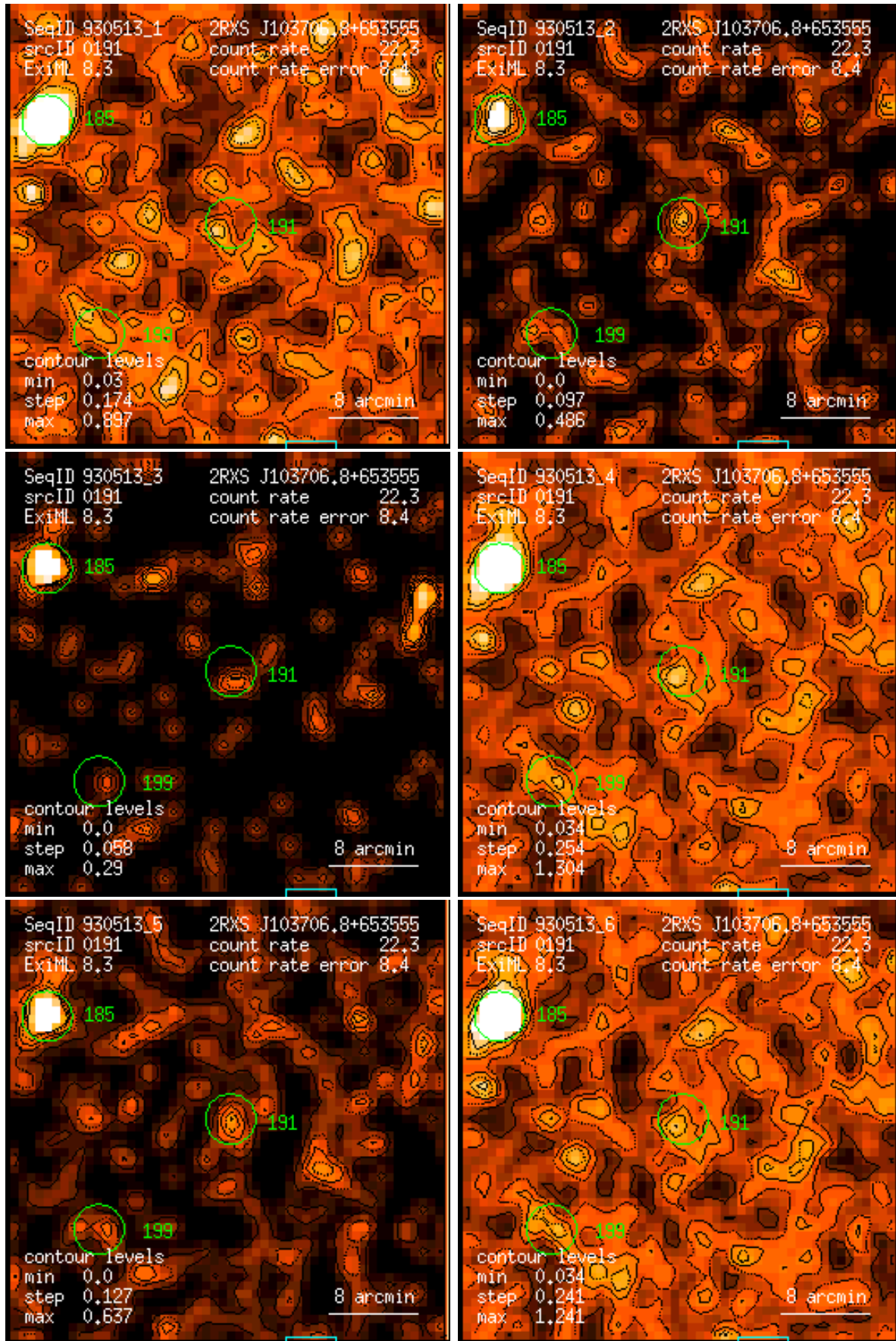
Figure 191: RASS 930513: detection 0191: band rate images, Gaussian filter: (1) PSPC channels 11 – 41, (2) 52 – 90, (3) 91 – 201, (4) 11 – 235, (5) 52 – 201, (6) 11 – 201. Broad band rates in counts/ks. Band rate contour levels in counts/ks/arcmin 2 .
