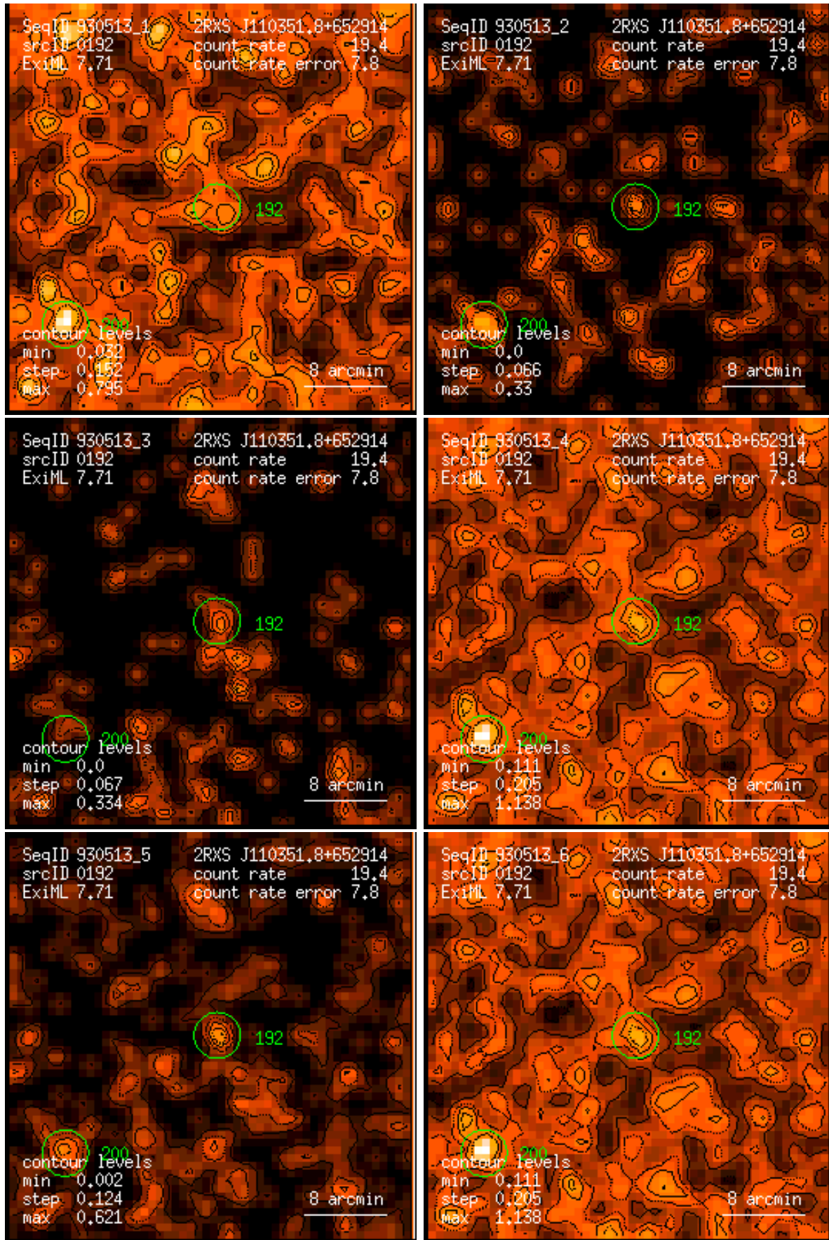
Figure 192: RASS 930513: detection 0192: band rate images, Gaussian filter: (1) PSPC channels 11 – 41, (2) 52 – 90, (3) 91 – 201, (4) 11 – 235, (5) 52 – 201, (6) 11 – 201. Broad band rates in counts/ks. Band rate contour levels in counts/ks/arcmin 2 .
