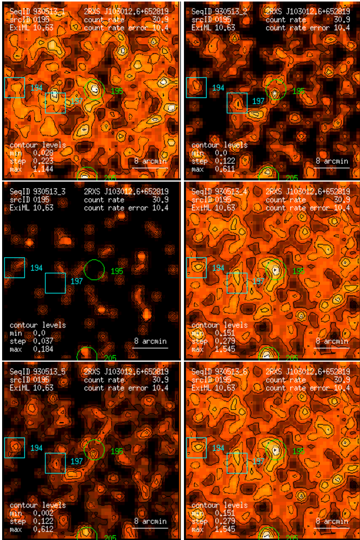
Figure 195: RASS 930513: detection 0195: band rate images, Gaussian filter: (1) PSPC channels 11 – 41, (2) 52 – 90, (3) 91 – 201, (4) 11 – 235, (5) 52 – 201, (6) 11 – 201. Broad band rates in counts/ks. Band rate contour levels in counts/ks/arcmin 2 .
