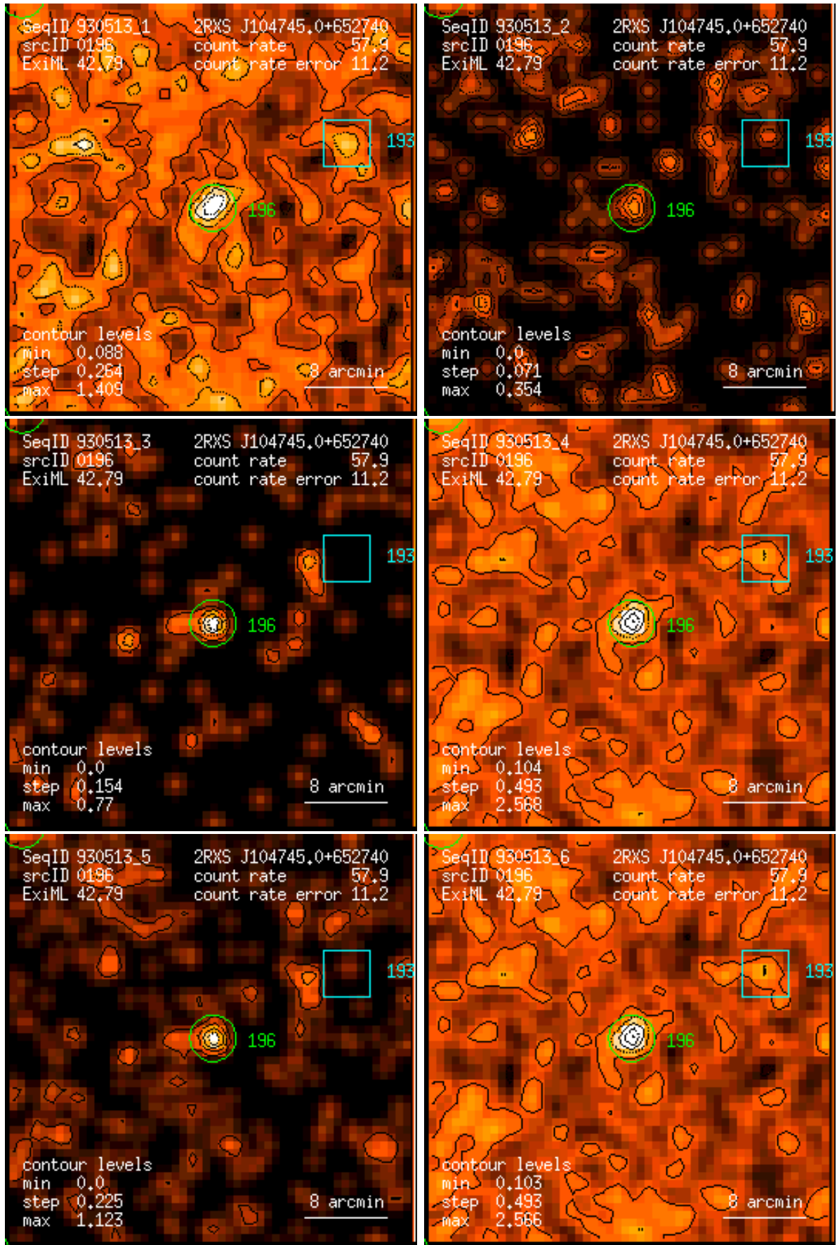
Figure 196: RASS 930513: detection 0196: band rate images, Gaussian filter: (1) PSPC channels 11 – 41, (2) 52 – 90, (3) 91 – 201, (4) 11 – 235, (5) 52 – 201, (6) 11 – 201. Broad band rates in counts/ks. Band rate contour levels in counts/ks/arcmin 2 .
