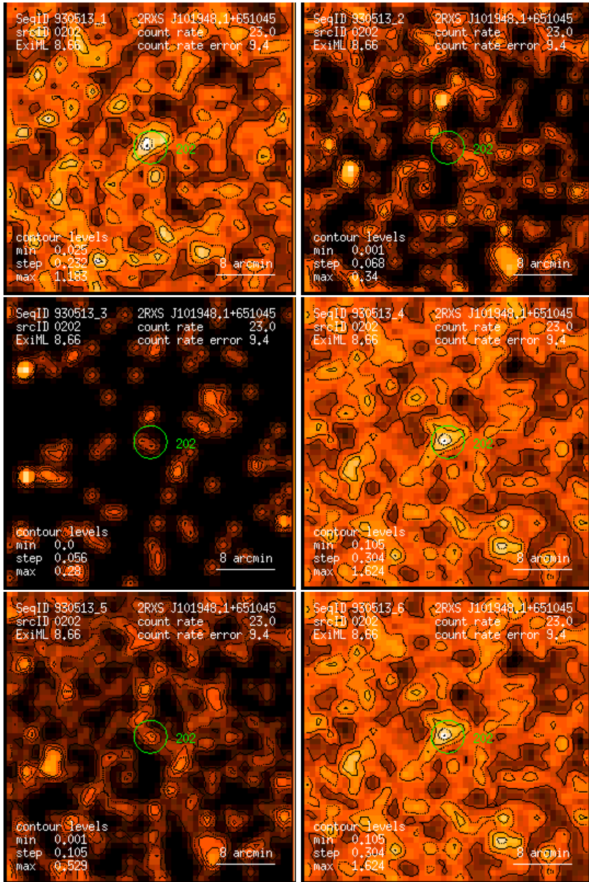
Figure 202: RASS 930513: detection 0202: band rate images, Gaussian filter: (1) PSPC channels 11 – 41, (2) 52 – 90, (3) 91 – 201, (4) 11 – 235, (5) 52 – 201, (6) 11 – 201. Broad band rates in counts/ks. Band rate contour levels in counts/ks/arcmin 2 .
