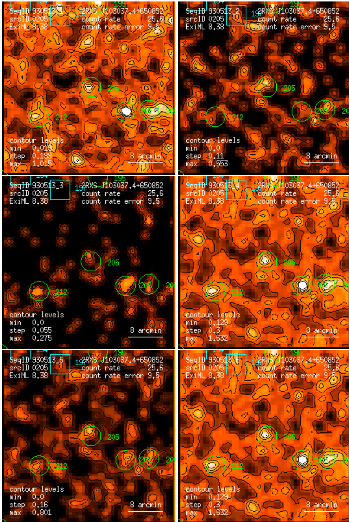
Figure 205: RASS 930513: detection 0205: band rate images, Gaussian filter: (1) PSPC channels 11 – 41, (2) 52 – 90, (3) 91 – 201, (4) 11 – 235, (5) 52 – 201, (6) 11 – 201. Broad band rates in counts/ks. Band rate contour levels in counts/ks/arcmin 2 .
