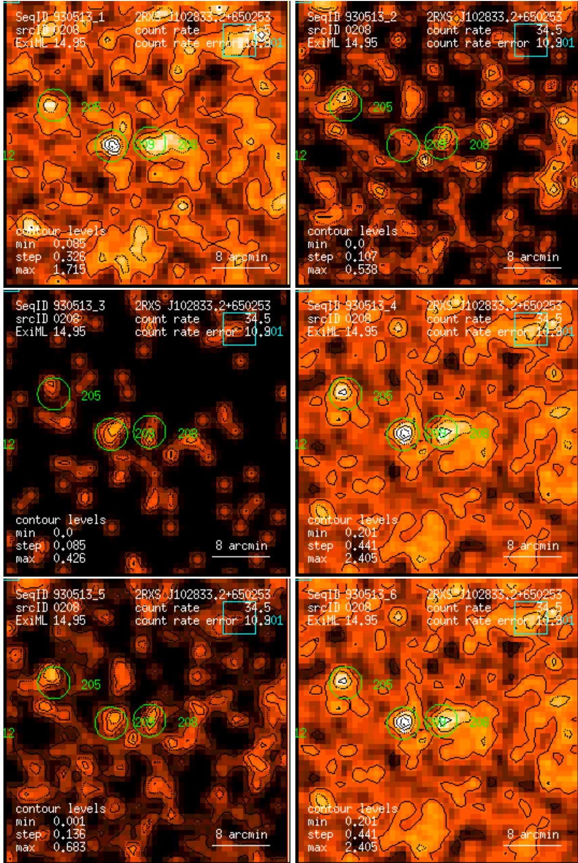
Figure 208: RASS 930513: detection 0208: band rate images, Gaussian filter: (1) PSPC channels 11 – 41, (2) 52 – 90, (3) 91 – 201, (4) 11 – 235, (5) 52 – 201, (6) 11 – 201. Broad band rates in counts/ks. Band rate contour levels in counts/ks/arcmin 2 .
