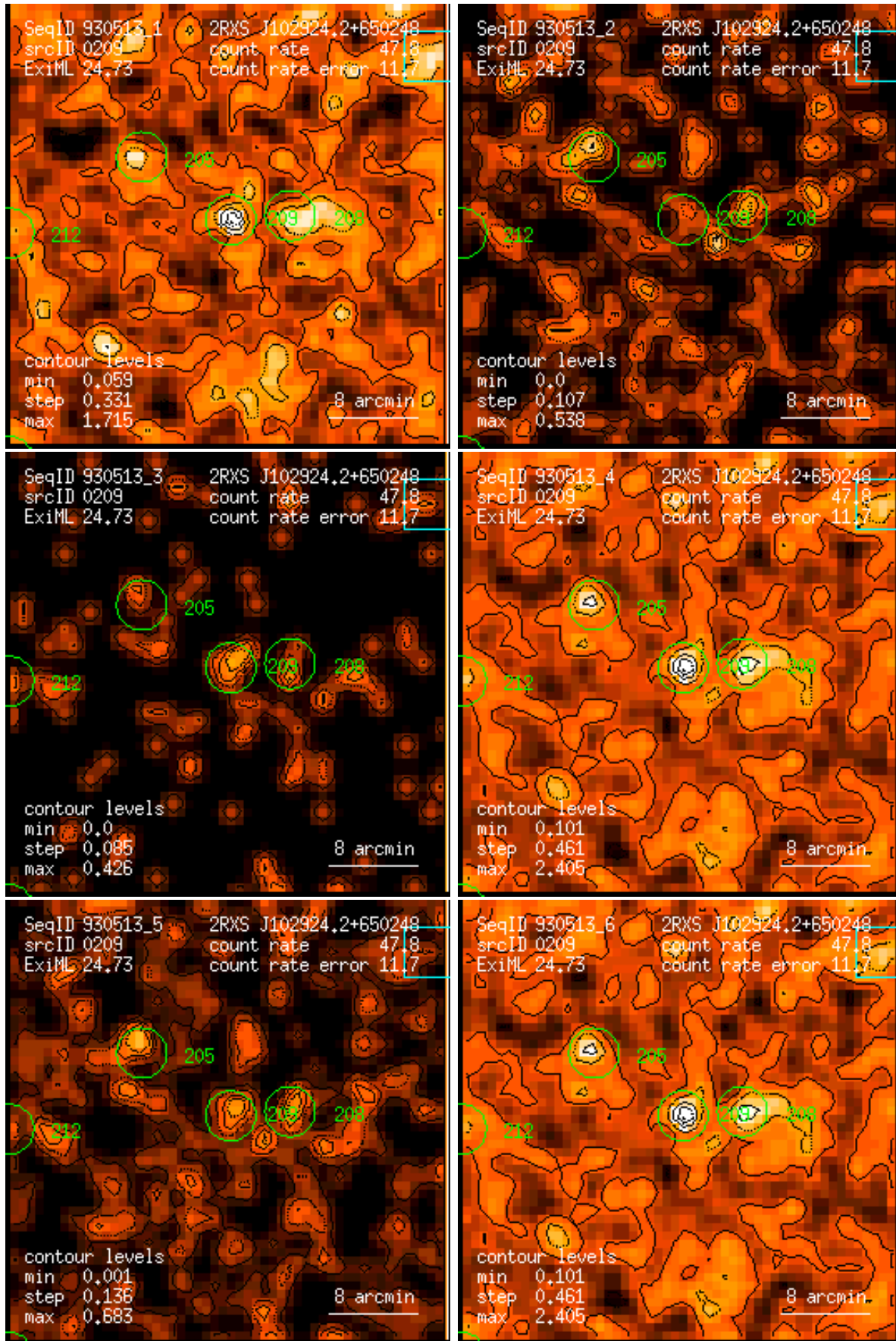
Figure 209: RASS 930513: detection 0209: band rate images, Gaussian filter: (1) PSPC channels 11 – 41, (2) 52 – 90, (3) 91 – 201, (4) 11 – 235, (5) 52 – 201, (6) 11 – 201. Broad band rates in counts/ks. Band rate contour levels in counts/ks/arcmin 2 .
