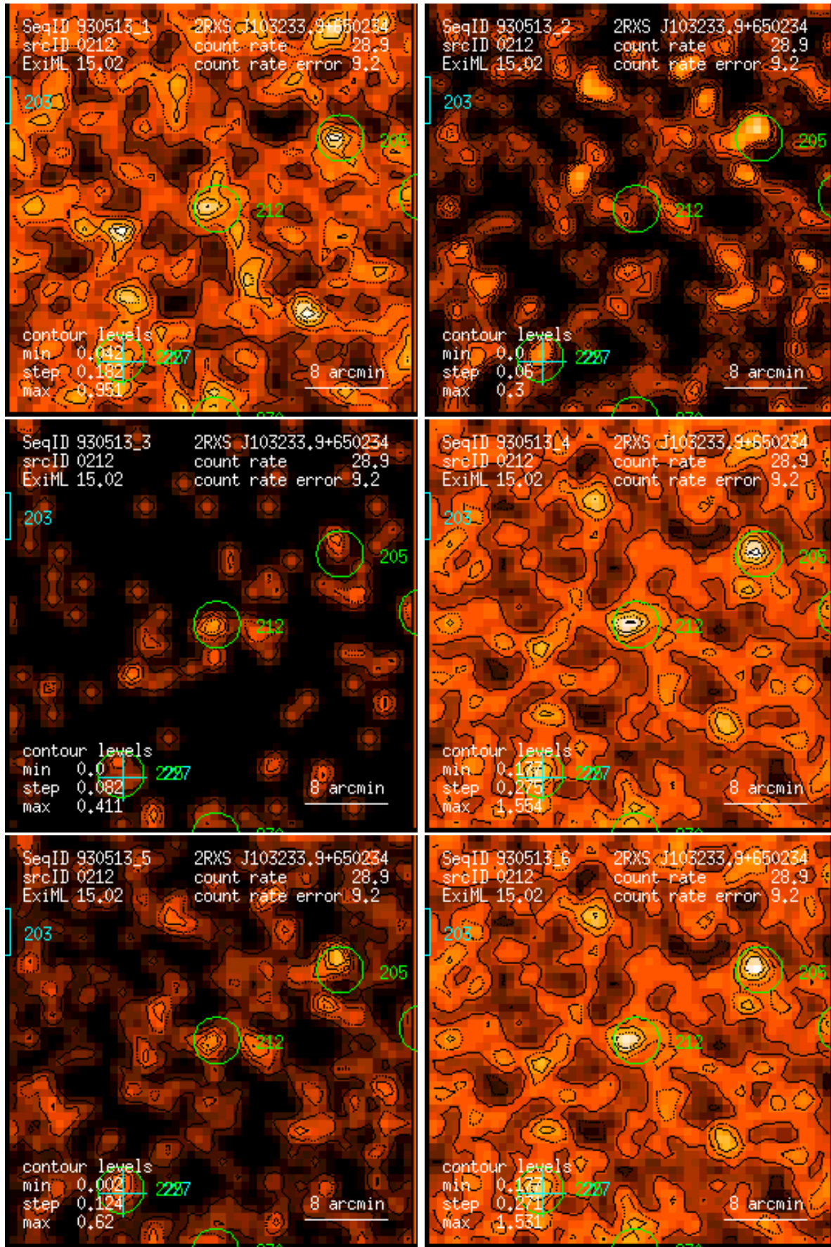
Figure 212: RASS 930513: detection 0212: band rate images, Gaussian filter: (1) PSPC channels 11 – 41, (2) 52 – 90, (3) 91 – 201, (4) 11 – 235, (5) 52 – 201, (6) 11 – 201. Broad band rates in counts/ks. Band rate contour levels in counts/ks/arcmin 2 .
