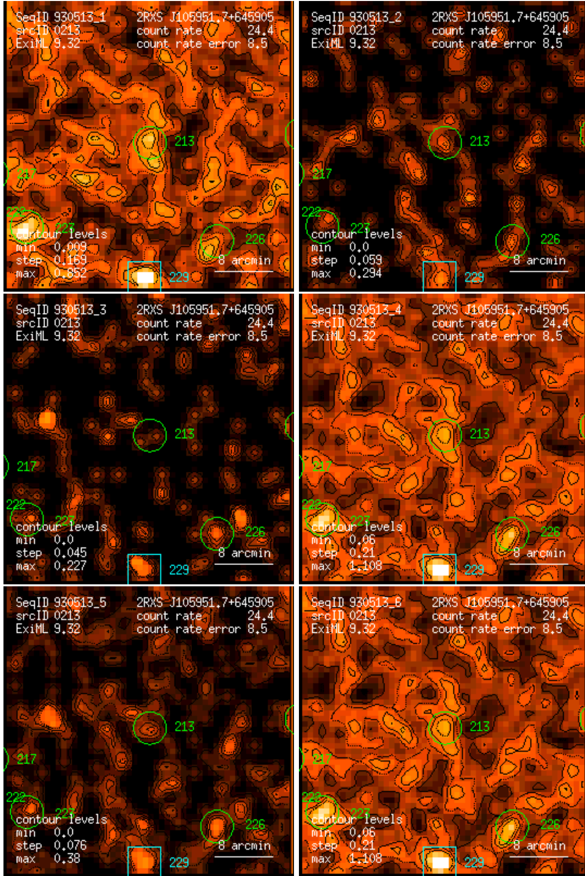
Figure 213: RASS 930513: detection 0213: band rate images, Gaussian filter: (1) PSPC channels 11 – 41, (2) 52 – 90, (3) 91 – 201, (4) 11 – 235, (5) 52 – 201, (6) 11 – 201. Broad band rates in counts/ks. Band rate contour levels in counts/ks/arcmin 2 .
