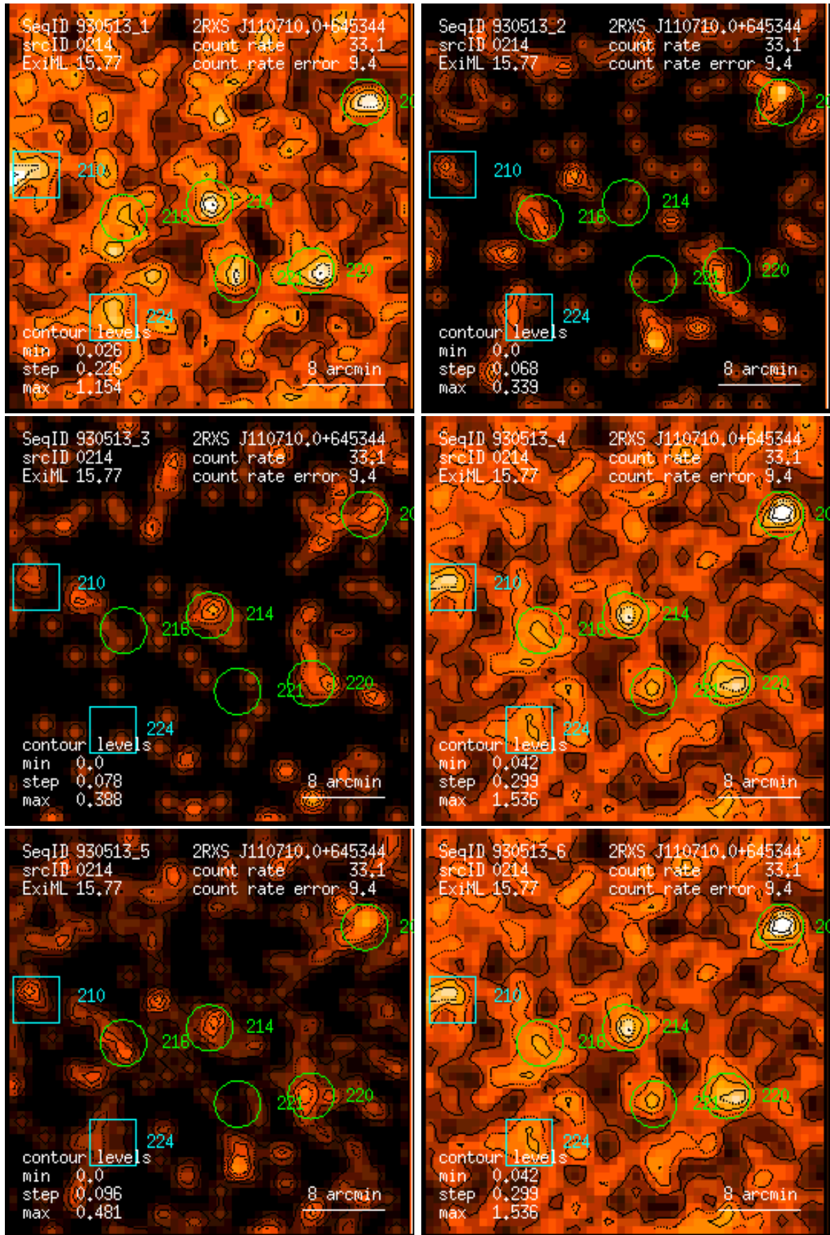
Figure 214: RASS 930513: detection 0214: band rate images, Gaussian filter: (1) PSPC channels 11 – 41, (2) 52 – 90, (3) 91 – 201, (4) 11 – 235, (5) 52 – 201, (6) 11 – 201. Broad band rates in counts/ks. Band rate contour levels in counts/ks/arcmin 2 .
