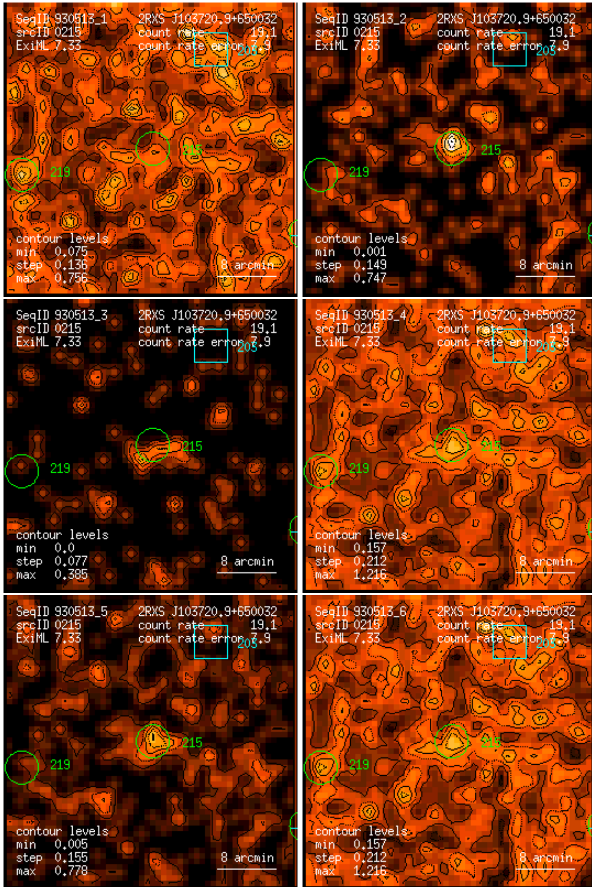
Figure 215: RASS 930513: detection 0215: band rate images, Gaussian filter: (1) PSPC channels 11 – 41, (2) 52 – 90, (3) 91 – 201, (4) 11 – 235, (5) 52 – 201, (6) 11 – 201. Broad band rates in counts/ks. Band rate contour levels in counts/ks/arcmin 2 .
