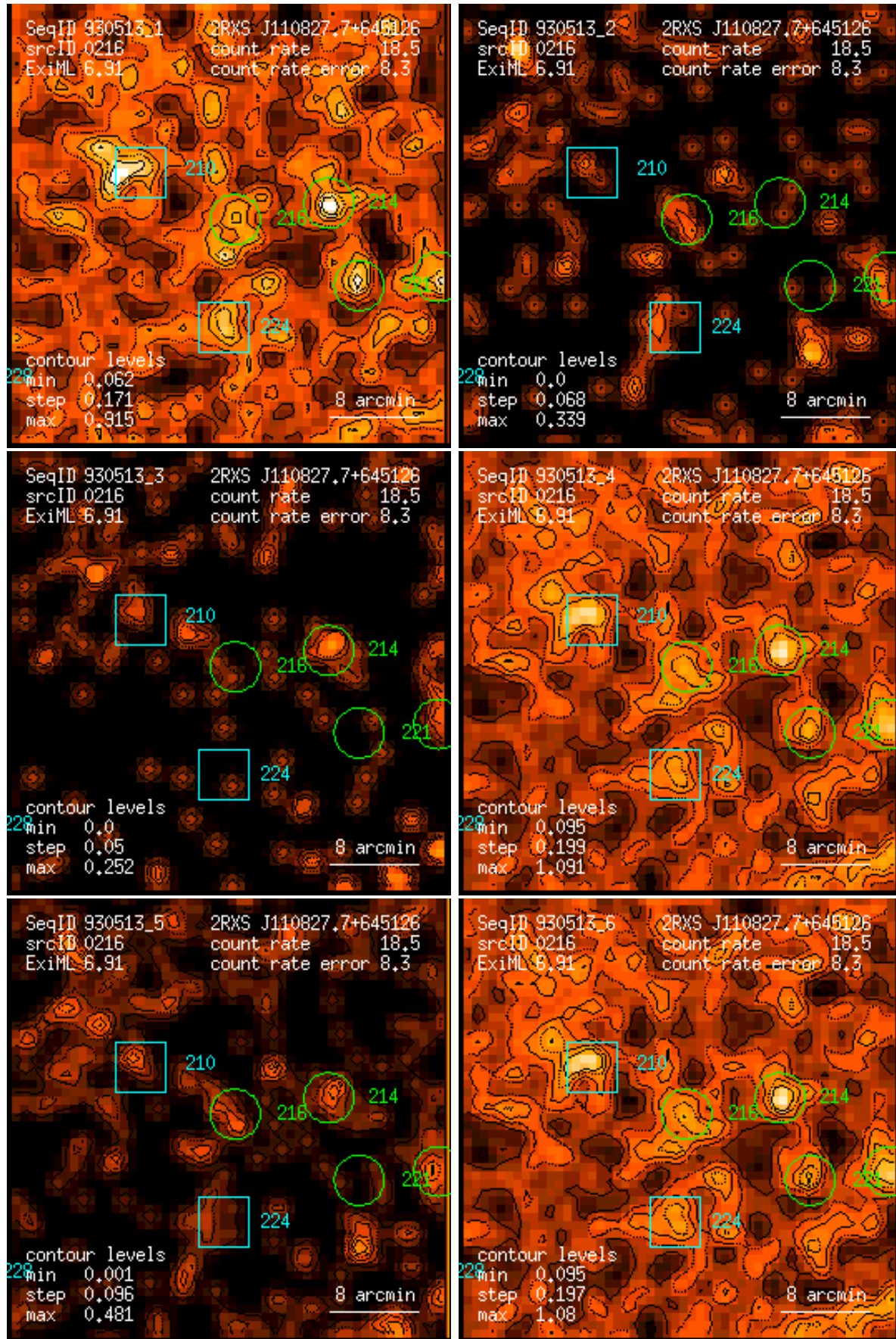
Figure 216: RASS 930513: detection 0216: band rate images, Gaussian filter: (1) PSPC channels 11 – 41, (2) 52 – 90, (3) 91 – 201, (4) 11 – 235, (5) 52 – 201, (6) 11 – 201. Broad band rates in counts/ks. Band rate contour levels in counts/ks/arcmin 2 .
