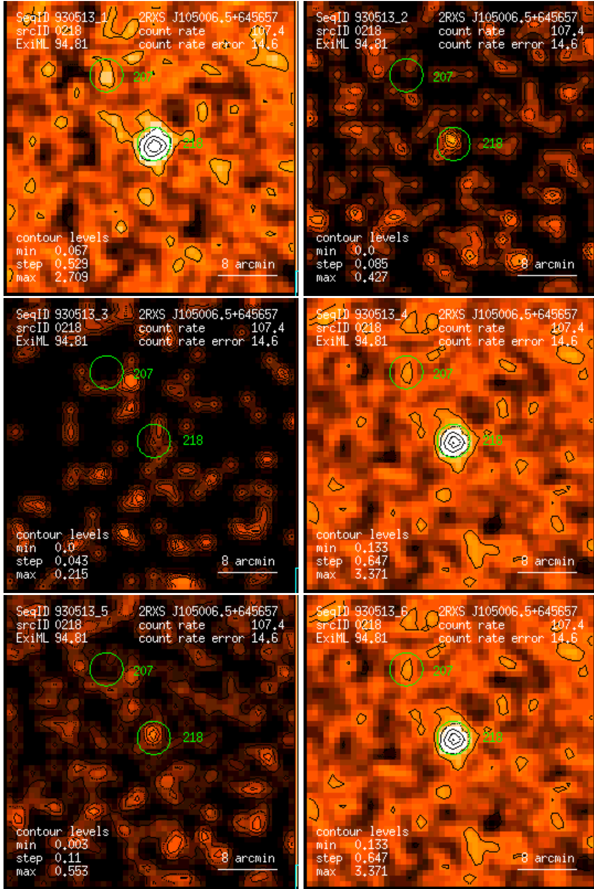
Figure 218: RASS 930513: detection 0218: band rate images, Gaussian filter: (1) PSPC channels 11 – 41, (2) 52 – 90, (3) 91 – 201, (4) 11 – 235, (5) 52 – 201, (6) 11 – 201. Broad band rates in counts/ks. Band rate contour levels in counts/ks/arcmin 2 .
