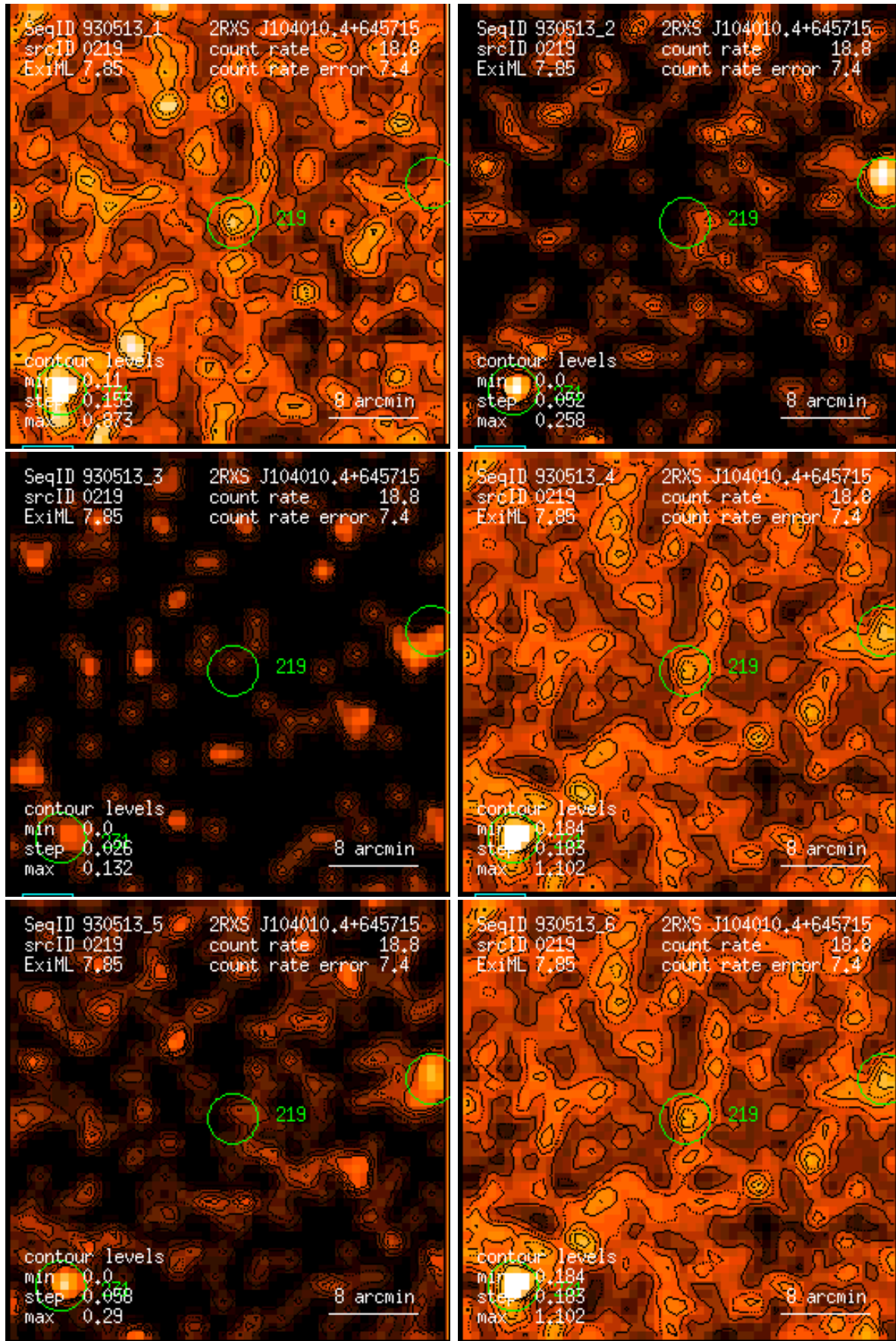
Figure 219: RASS 930513: detection 0219: band rate images, Gaussian filter: (1) PSPC channels 11 – 41, (2) 52 – 90, (3) 91 – 201, (4) 11 – 235, (5) 52 – 201, (6) 11 – 201. Broad band rates in counts/ks. Band rate contour levels in counts/ks/arcmin 2 .
