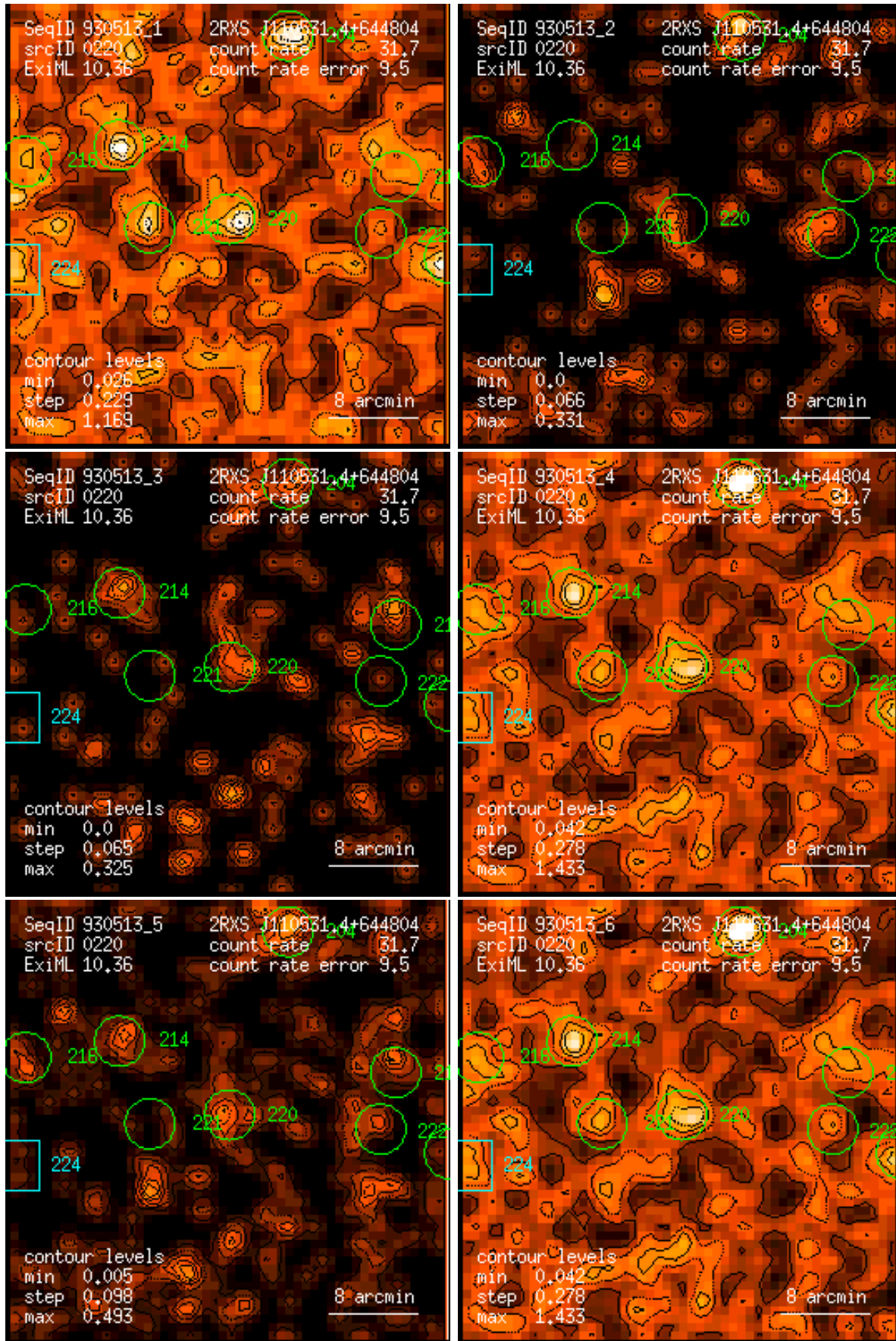
Figure 220: RASS 930513: detection 0220: band rate images, Gaussian filter: (1) PSPC channels 11 – 41, (2) 52 – 90, (3) 91 – 201, (4) 11 – 235, (5) 52 – 201, (6) 11 – 201. Broad band rates in counts/ks. Band rate contour levels in counts/ks/arcmin 2 .
