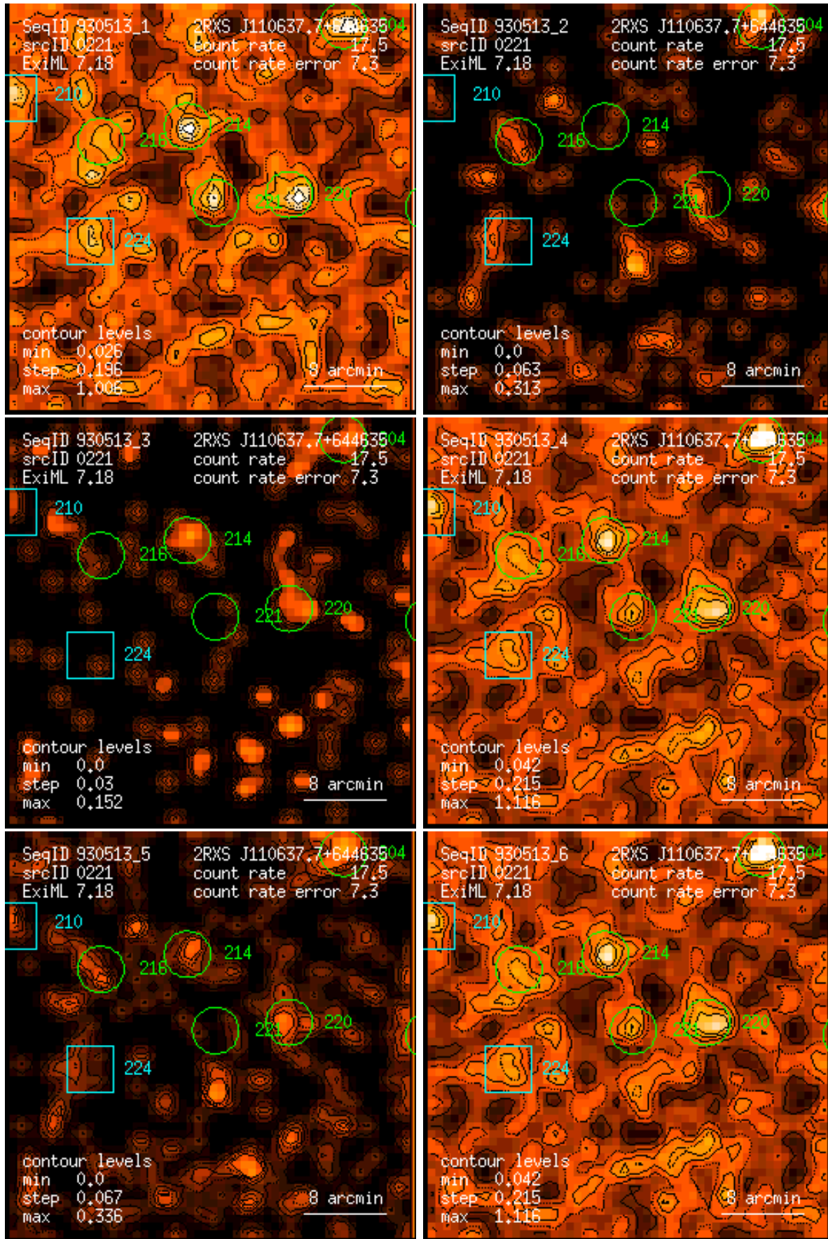
Figure 221: RASS 930513: detection 0221: band rate images, Gaussian filter: (1) PSPC channels 11 – 41, (2) 52 – 90, (3) 91 – 201, (4) 11 – 235, (5) 52 – 201, (6) 11 – 201. Broad band rates in counts/ks. Band rate contour levels in counts/ks/arcmin 2 .
