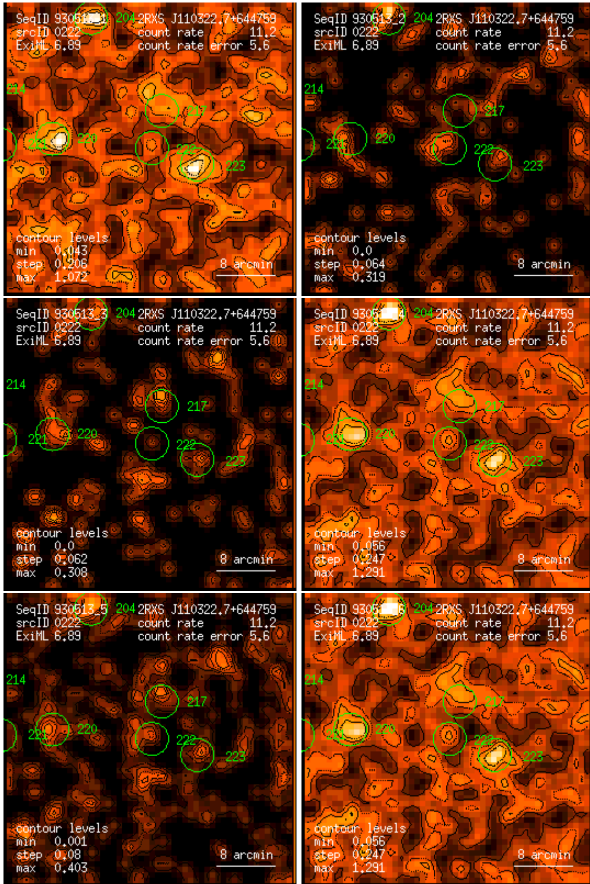
Figure 222: RASS 930513: detection 0222: band rate images, Gaussian filter: (1) PSPC channels 11 – 41, (2) 52 – 90, (3) 91 – 201, (4) 11 – 235, (5) 52 – 201, (6) 11 – 201. Broad band rates in counts/ks. Band rate contour levels in counts/ks/arcmin 2 .
