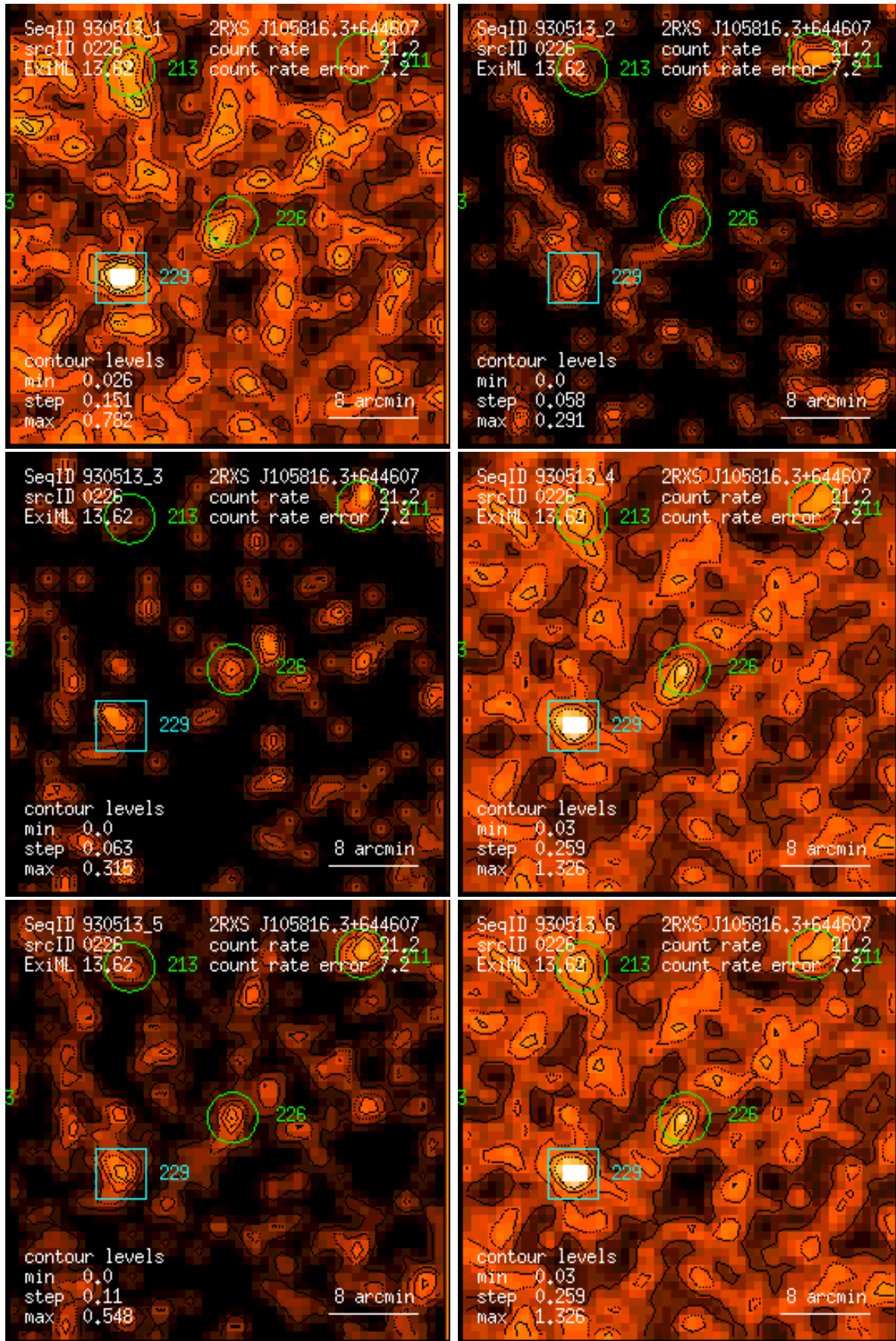
Figure 226: RASS 930513: detection 0226: band rate images, Gaussian filter: (1) PSPC channels 11 – 41, (2) 52 – 90, (3) 91 – 201, (4) 11 – 235, (5) 52 – 201, (6) 11 – 201. Broad band rates in counts/ks. Band rate contour levels in counts/ks/arcmin 2 .
