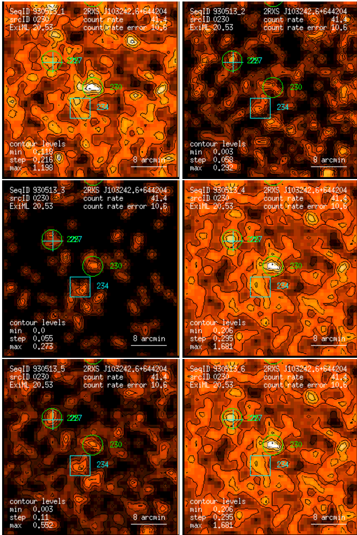
Figure 230: RASS 930513: detection 0230: band rate images, Gaussian filter: (1) PSPC channels 11 – 41, (2) 52 – 90, (3) 91 – 201, (4) 11 – 235, (5) 52 – 201, (6) 11 – 201. Broad band rates in counts/ks. Band rate contour levels in counts/ks/arcmin 2 .
