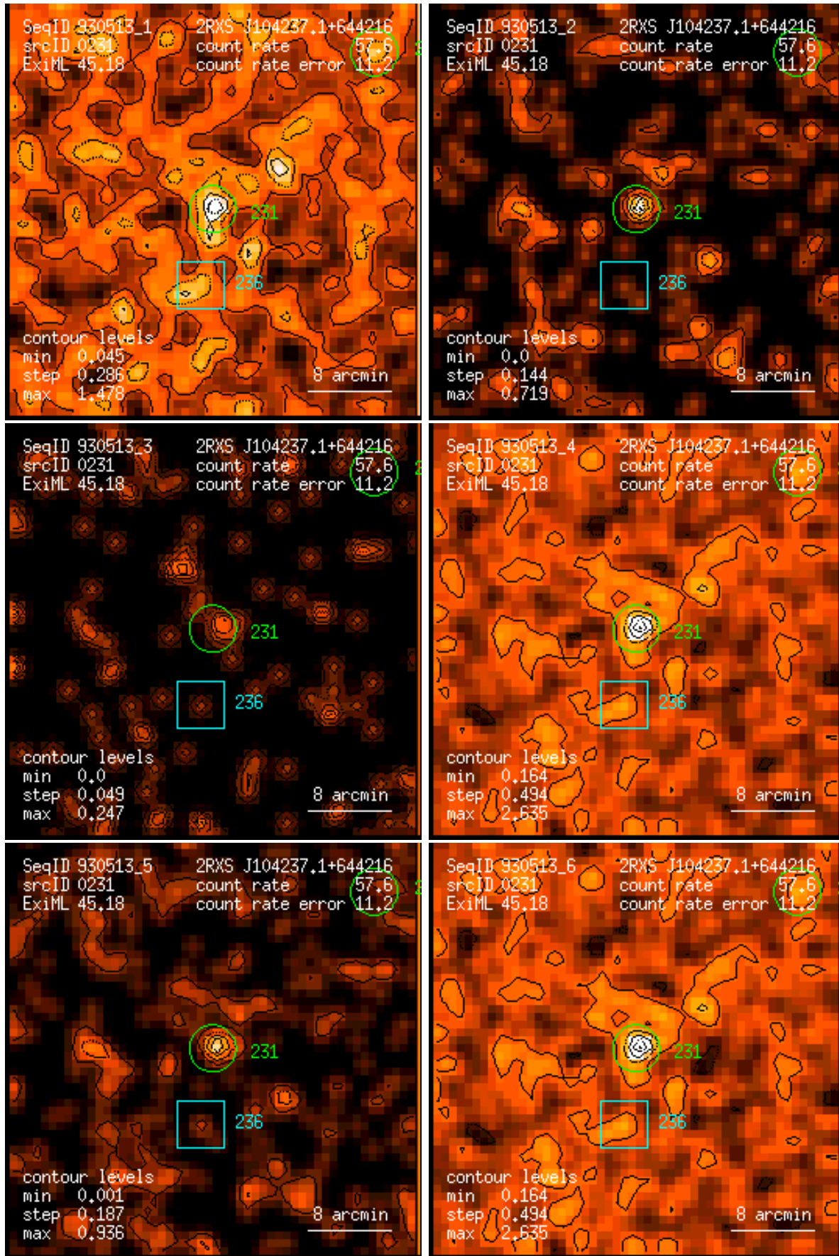
Figure 231: RASS 930513: detection 0231: band rate images, Gaussian filter: (1) PSPC channels 11 – 41, (2) 52 – 90, (3) 91 – 201, (4) 11 – 235, (5) 52 – 201, (6) 11 – 201. Broad band rates in counts/ks. Band rate contour levels in counts/ks/arcmin 2 .
