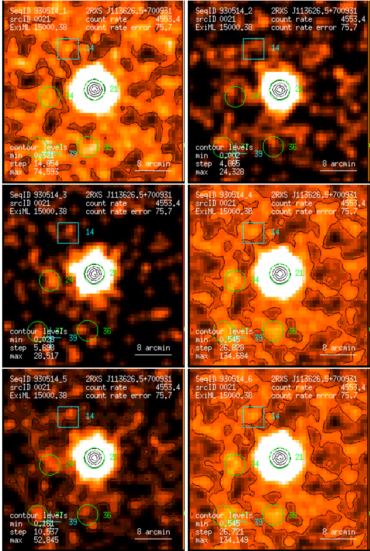
Figure 21: RASS 930514: detection 0021: band rate images, Gaussian filter: (1) PSPC channels 11 – 41, (2) 52 – 90, (3) 91 – 201, (4) 11 – 235, (5) 52 – 201, (6) 11 – 201. Broad band rates in counts/ks. Band rate contour levels in counts/ks/arcmin 2 .
