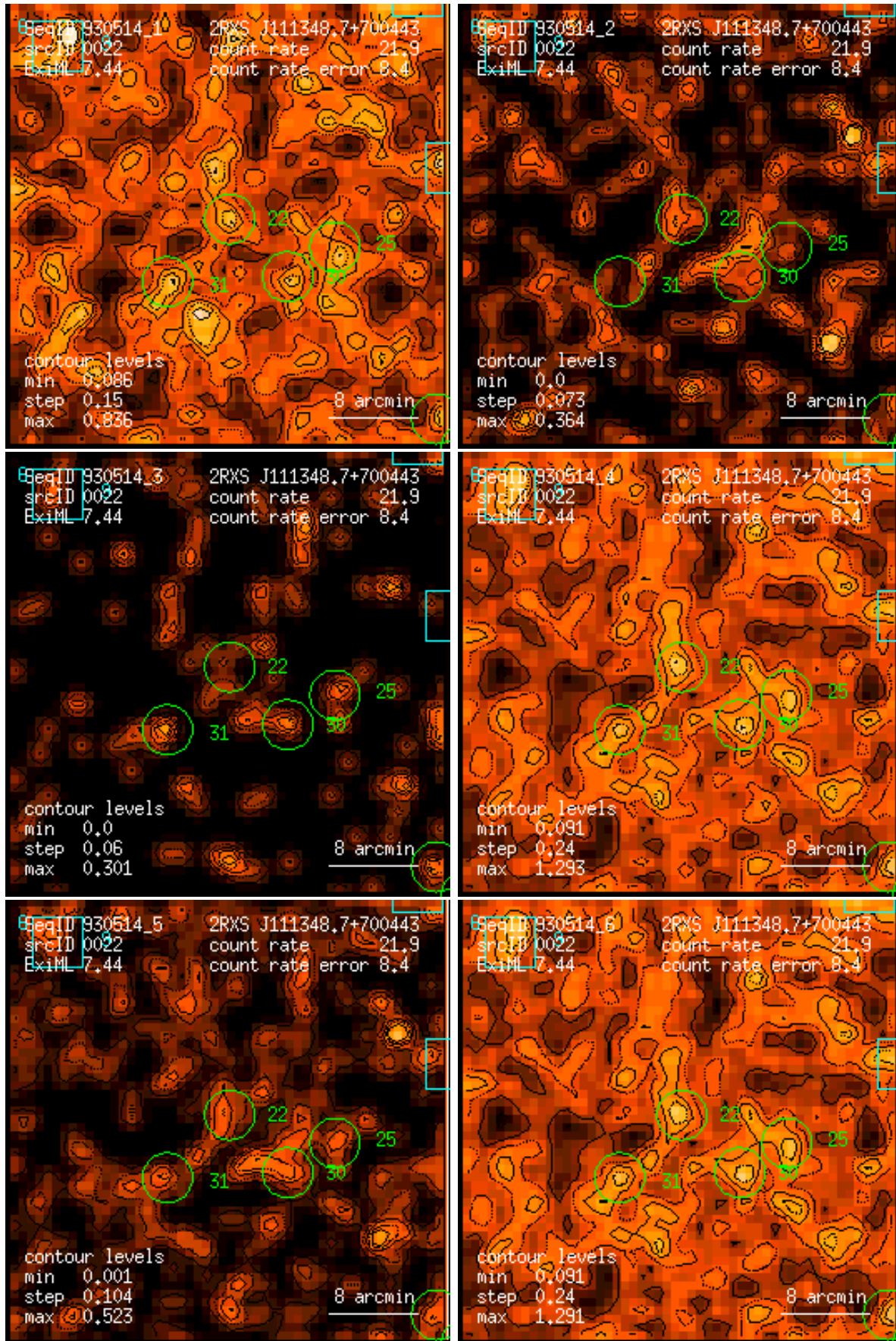
Figure 22: RASS 930514: detection 0022: band rate images, Gaussian filter: (1) PSPC channels 11 – 41, (2) 52 – 90, (3) 91 – 201, (4) 11 – 235, (5) 52 – 201, (6) 11 – 201. Broad band rates in counts/ks. Band rate contour levels in counts/ks/arcmin 2 .
